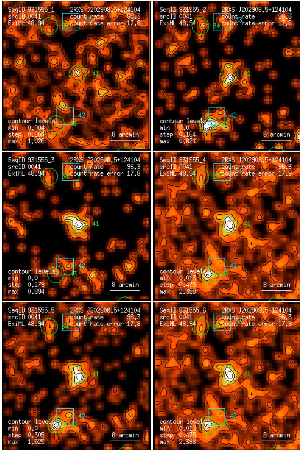
Figure 41: RASS 931555: detection 0041: band rate images, Gaussian filter: (1) PSPC channels 11 – 41, (2) 52 – 90, (3) 91 – 201, (4) 11 – 235, (5) 52 – 201, (6) 11 – 201. Broad band rates in counts/ks. Band rate contour levels in counts/ks/arcmin 2 .
