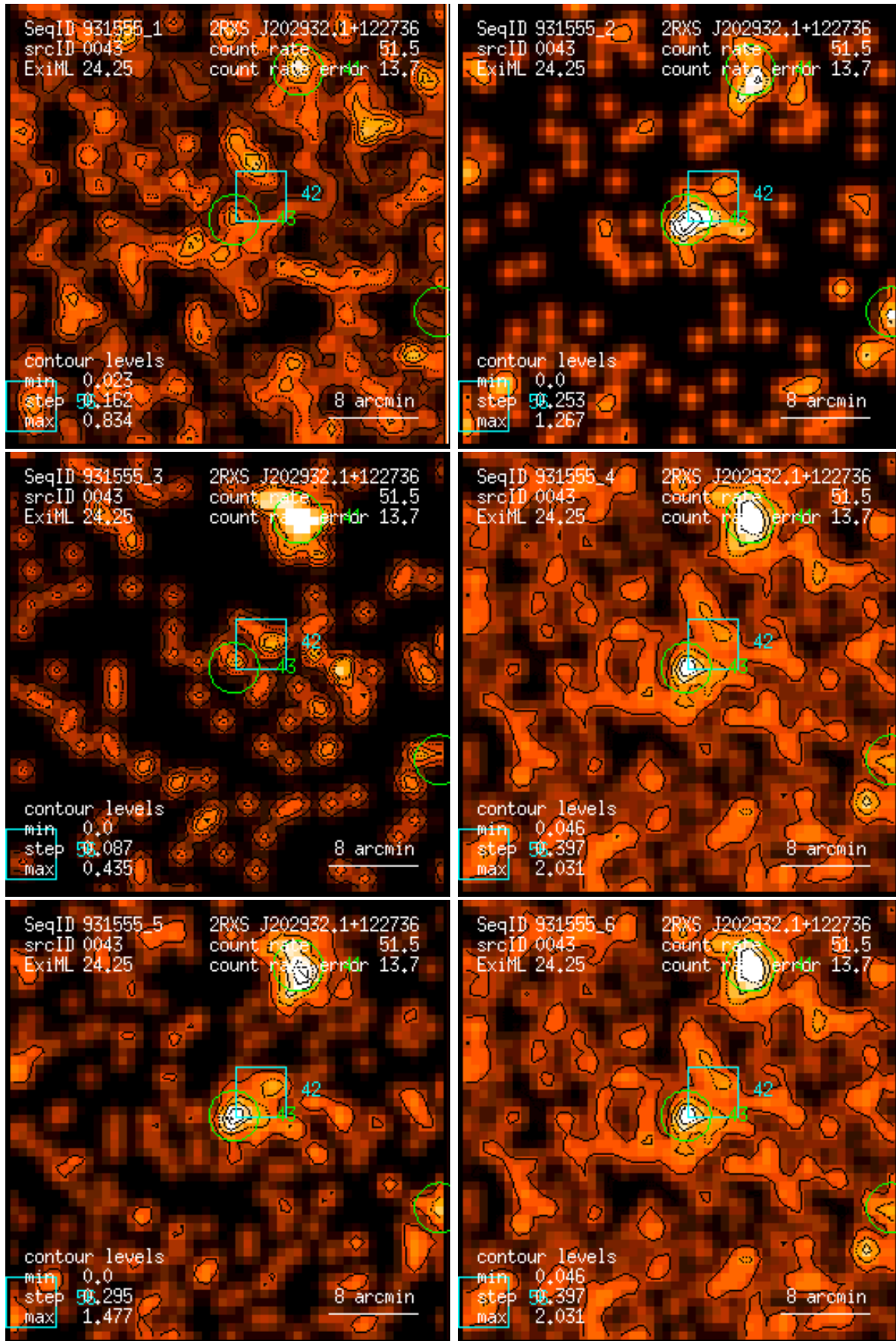
Figure 43: RASS 931555: detection 0043: band rate images, Gaussian filter: (1) PSPC channels 11 – 41, (2) 52 – 90, (3) 91 – 201, (4) 11 – 235, (5) 52 – 201, (6) 11 – 201. Broad band rates in counts/ks. Band rate contour levels in counts/ks/arcmin 2 .
