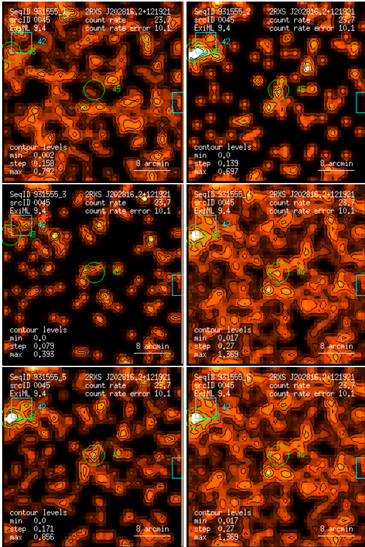
Figure 45: RASS 931555: detection 0045: band rate images, Gaussian filter: (1) PSPC channels 11 – 41, (2) 52 – 90, (3) 91 – 201, (4) 11 – 235, (5) 52 – 201, (6) 11 – 201. Broad band rates in counts/ks. Band rate contour levels in counts/ks/arcmin 2 .
