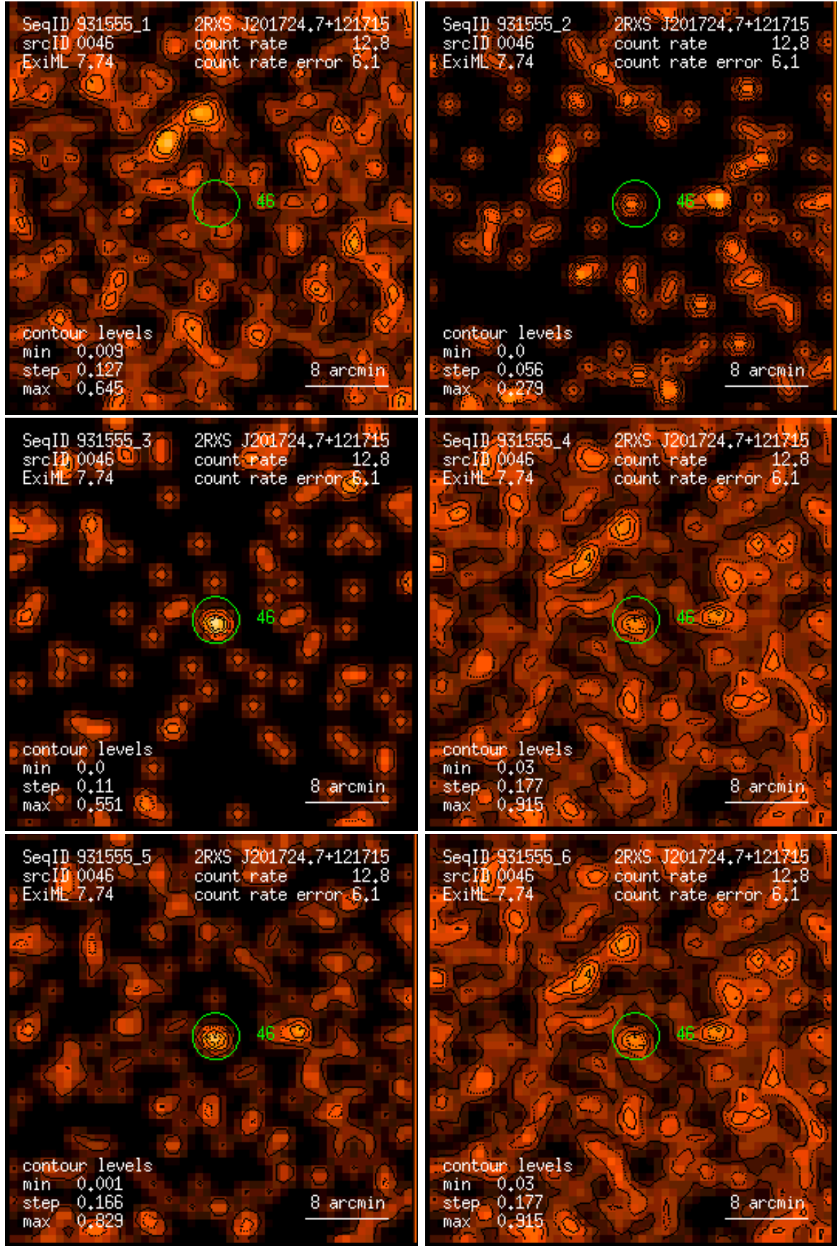
Figure 46: RASS 931555: detection 0046: band rate images, Gaussian filter: (1) PSPC channels 11 – 41, (2) 52 – 90, (3) 91 – 201, (4) 11 – 235, (5) 52 – 201, (6) 11 – 201. Broad band rates in counts/ks. Band rate contour levels in counts/ks/arcmin 2 .
