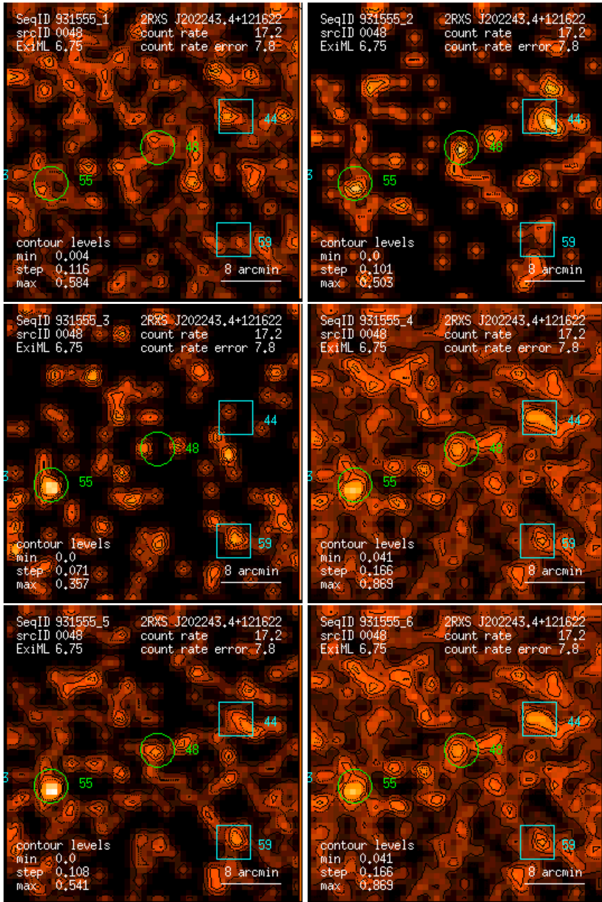
Figure 48: RASS 931555: detection 0048: band rate images, Gaussian filter: (1) PSPC channels 11 – 41, (2) 52 – 90, (3) 91 – 201, (4) 11 – 235, (5) 52 – 201, (6) 11 – 201. Broad band rates in counts/ks. Band rate contour levels in counts/ks/arcmin 2 .
