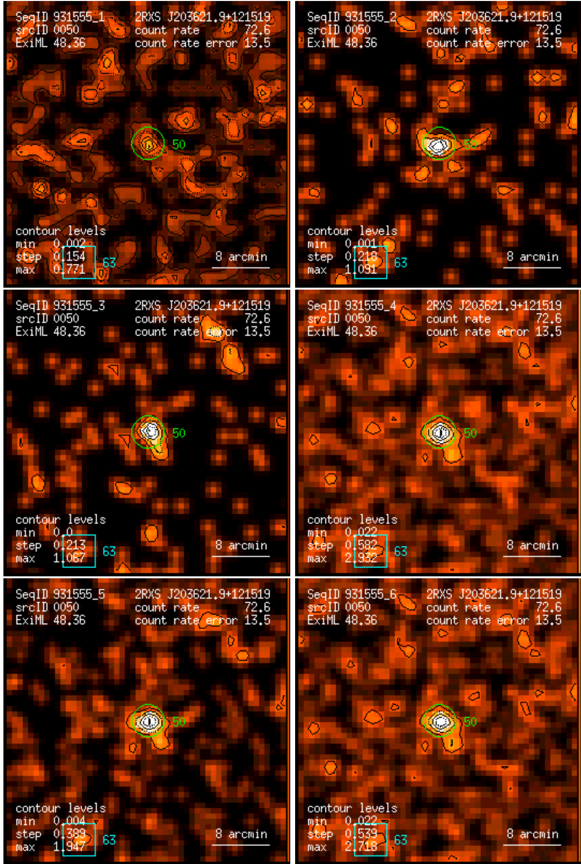
Figure 50: RASS 931555: detection 0050: band rate images, Gaussian filter: (1) PSPC channels 11 – 41, (2) 52 – 90, (3) 91 – 201, (4) 11 – 235, (5) 52 – 201, (6) 11 – 201. Broad band rates in counts/ks. Band rate contour levels in counts/ks/arcmin 2 .
