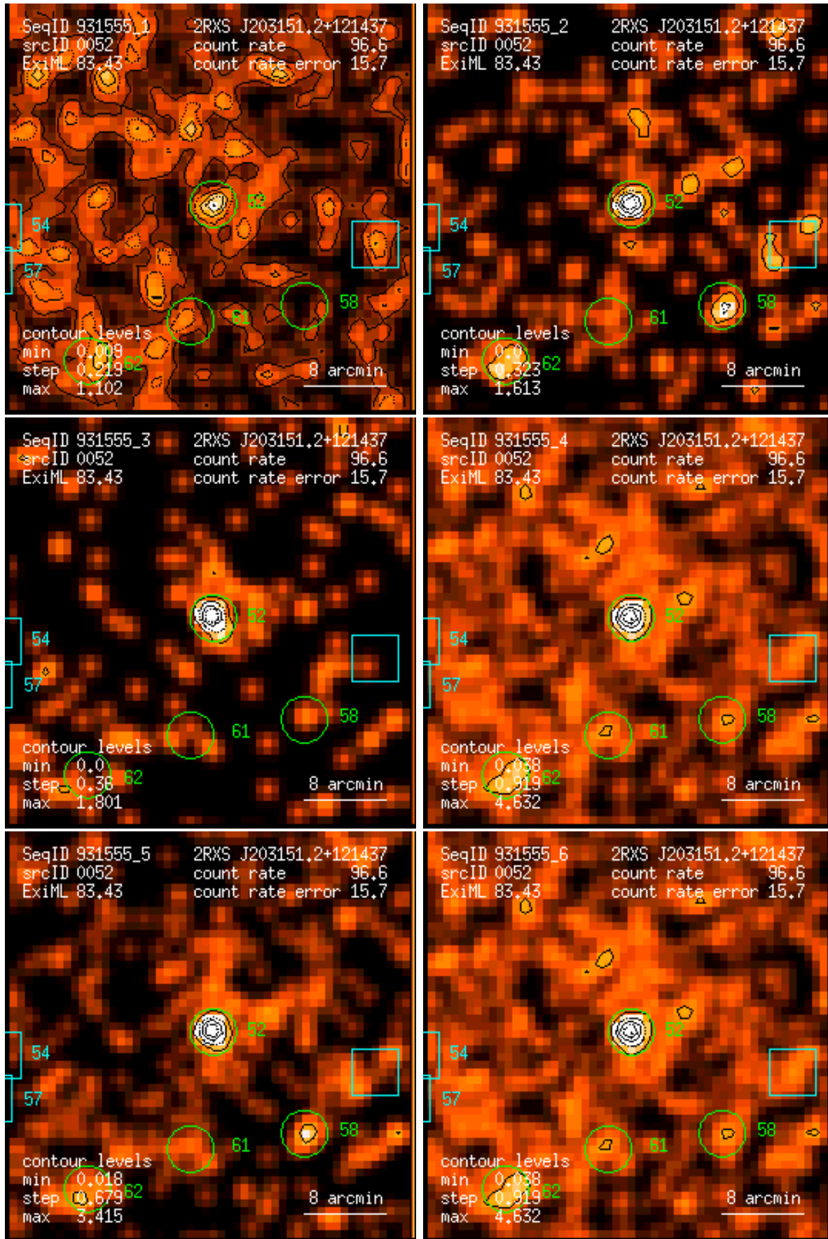
Figure 52: RASS 931555: detection 0052: band rate images, Gaussian filter: (1) PSPC channels 11 – 41, (2) 52 – 90, (3) 91 – 201, (4) 11 – 235, (5) 52 – 201, (6) 11 – 201. Broad band rates in counts/ks. Band rate contour levels in counts/ks/arcmin 2 .
