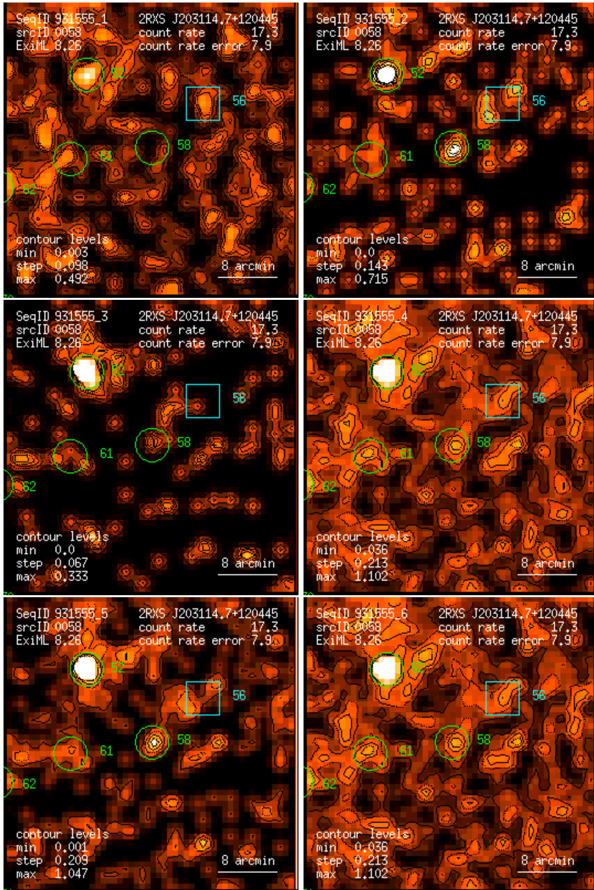
Figure 58: RASS 931555: detection 0058: band rate images, Gaussian filter: (1) PSPC channels 11 – 41, (2) 52 – 90, (3) 91 – 201, (4) 11 – 235, (5) 52 – 201, (6) 11 – 201. Broad band rates in counts/ks. Band rate contour levels in counts/ks/arcmin 2 .
