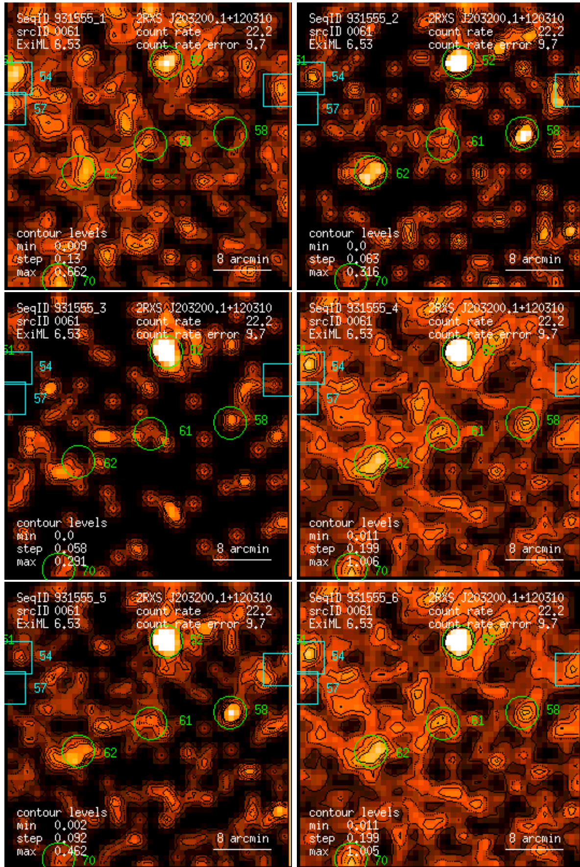
Figure 61: RASS 931555: detection 0061: band rate images, Gaussian filter: (1) PSPC channels 11 – 41, (2) 52 – 90, (3) 91 – 201, (4) 11 – 235, (5) 52 – 201, (6) 11 – 201. Broad band rates in counts/ks. Band rate contour levels in counts/ks/arcmin 2 .
