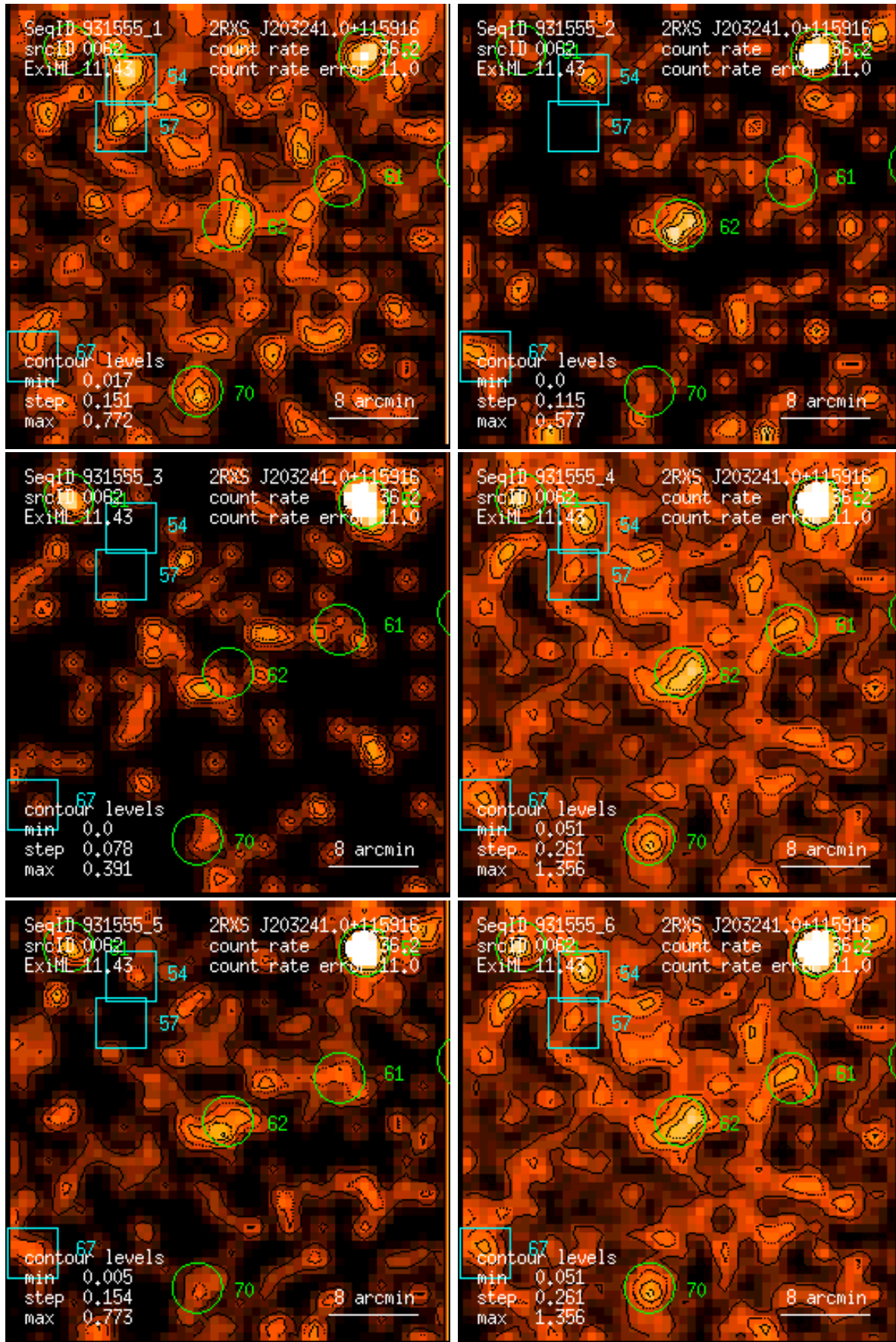
Figure 62: RASS 931555: detection 0062: band rate images, Gaussian filter: (1) PSPC channels 11 – 41, (2) 52 – 90, (3) 91 – 201, (4) 11 – 235, (5) 52 – 201, (6) 11 – 201. Broad band rates in counts/ks. Band rate contour levels in counts/ks/arcmin 2 .
