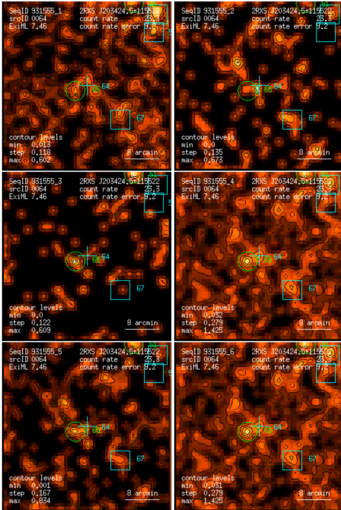
Figure 64: RASS 931555: detection 0064: band rate images, Gaussian filter: (1) PSPC channels 11 – 41, (2) 52 – 90, (3) 91 – 201, (4) 11 – 235, (5) 52 – 201, (6) 11 – 201. Broad band rates in counts/ks. Band rate contour levels in counts/ks/arcmin 2 .
