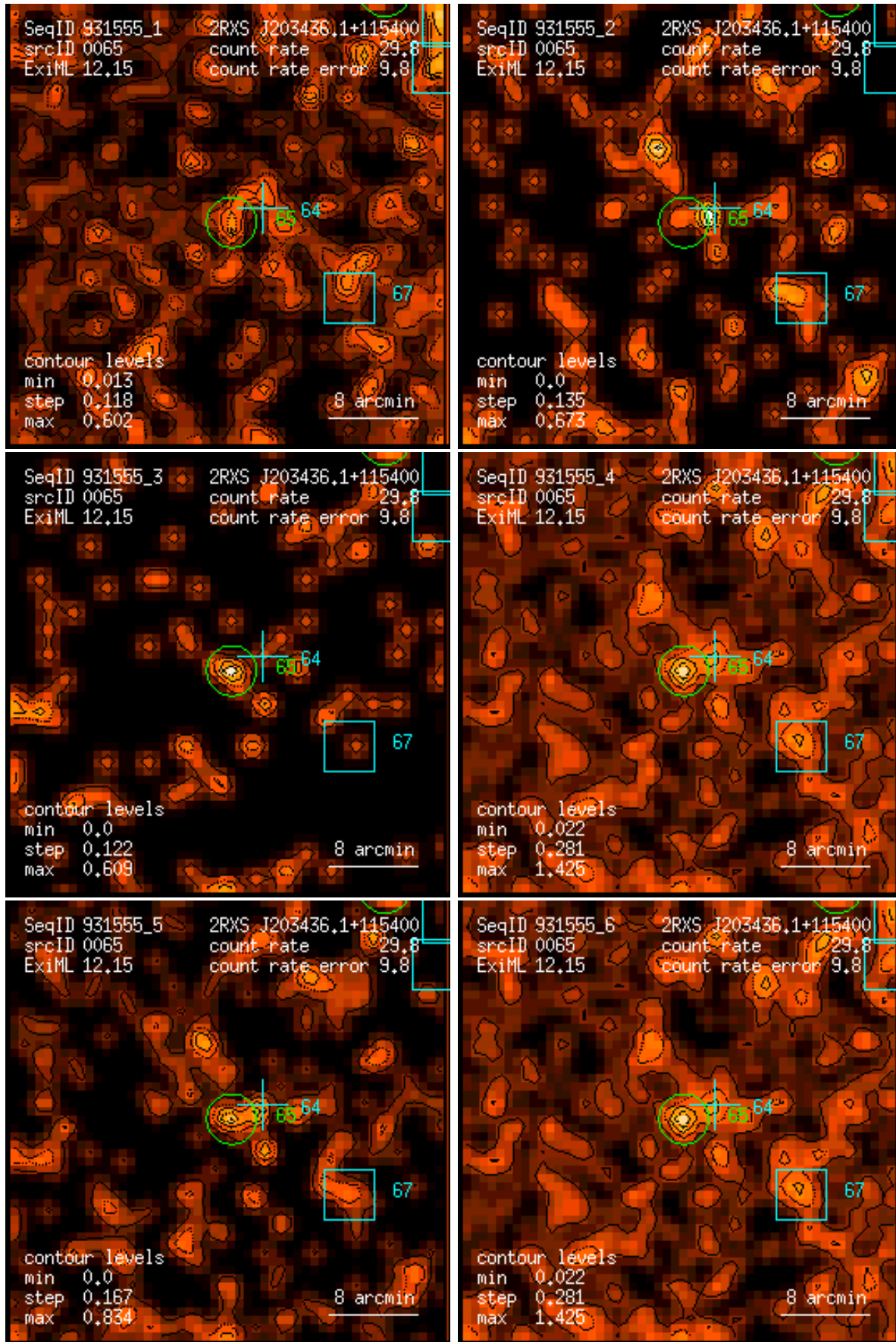
Figure 65: RASS 931555: detection 0065: band rate images, Gaussian filter: (1) PSPC channels 11 – 41, (2) 52 – 90, (3) 91 – 201, (4) 11 – 235, (5) 52 – 201, (6) 11 – 201. Broad band rates in counts/ks. Band rate contour levels in counts/ks/arcmin 2 .
