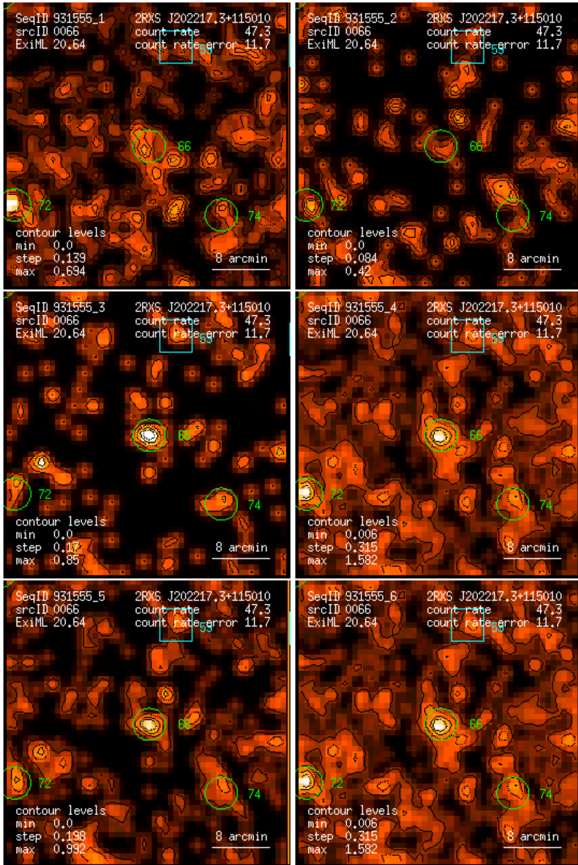
Figure 66: RASS 931555: detection 0066: band rate images, Gaussian filter: (1) PSPC channels 11 – 41, (2) 52 – 90, (3) 91 – 201, (4) 11 – 235, (5) 52 – 201, (6) 11 – 201. Broad band rates in counts/ks. Band rate contour levels in counts/ks/arcmin 2 .
