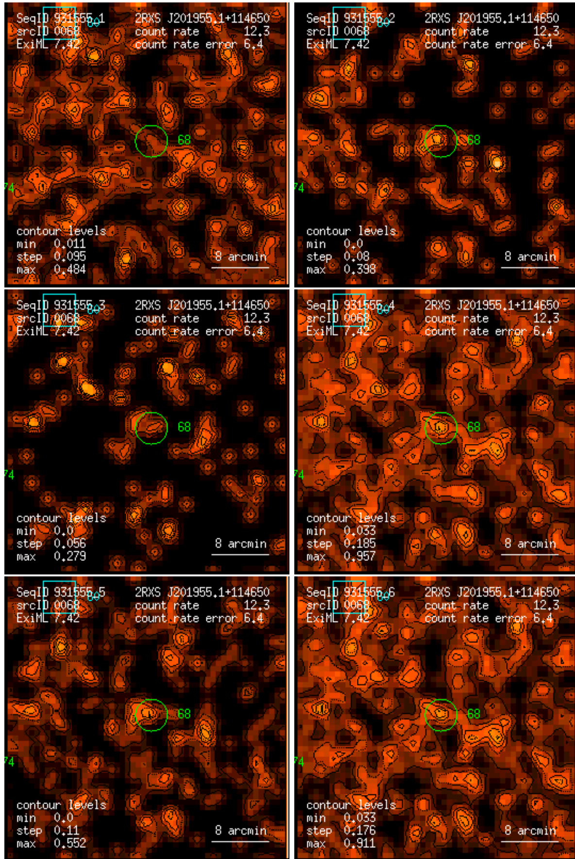
Figure 68: RASS 931555: detection 0068: band rate images, Gaussian filter: (1) PSPC channels 11 – 41, (2) 52 – 90, (3) 91 – 201, (4) 11 – 235, (5) 52 – 201, (6) 11 – 201. Broad band rates in counts/ks. Band rate contour levels in counts/ks/arcmin 2 .
