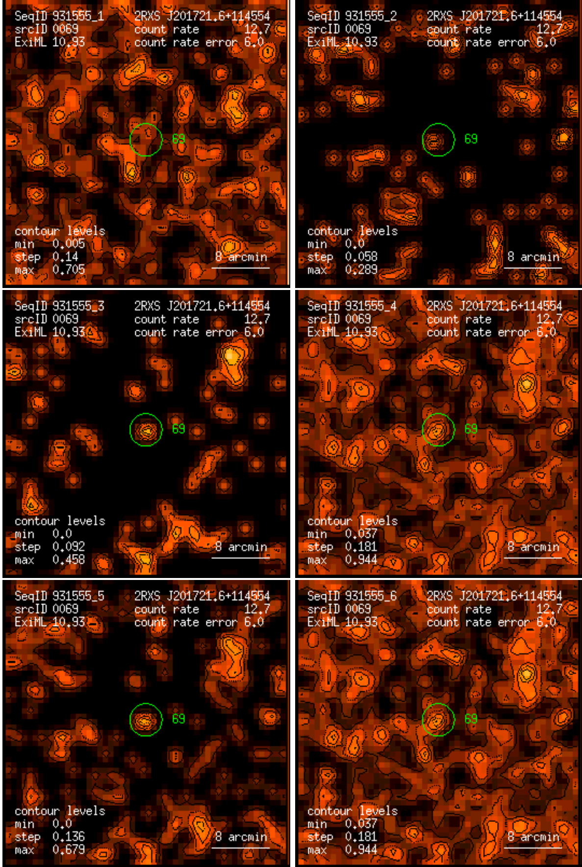
Figure 69: RASS 931555: detection 0069: band rate images, Gaussian filter: (1) PSPC channels 11 – 41, (2) 52 – 90, (3) 91 – 201, (4) 11 – 235, (5) 52 – 201, (6) 11 – 201. Broad band rates in counts/ks. Band rate contour levels in counts/ks/arcmin 2 .
