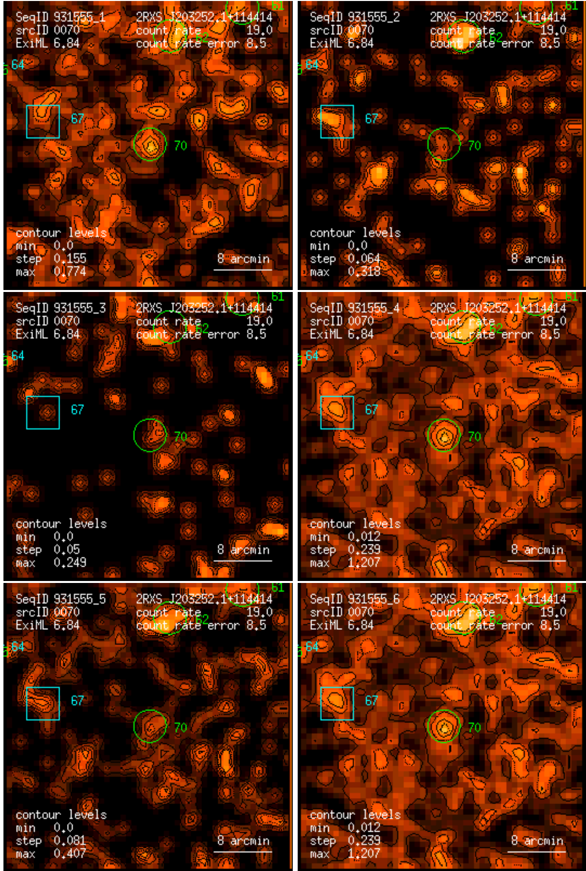
Figure 70: RASS 931555: detection 0070: band rate images, Gaussian filter: (1) PSPC channels 11 – 41, (2) 52 – 90, (3) 91 – 201, (4) 11 – 235, (5) 52 – 201, (6) 11 – 201. Broad band rates in counts/ks. Band rate contour levels in counts/ks/arcmin 2 .
