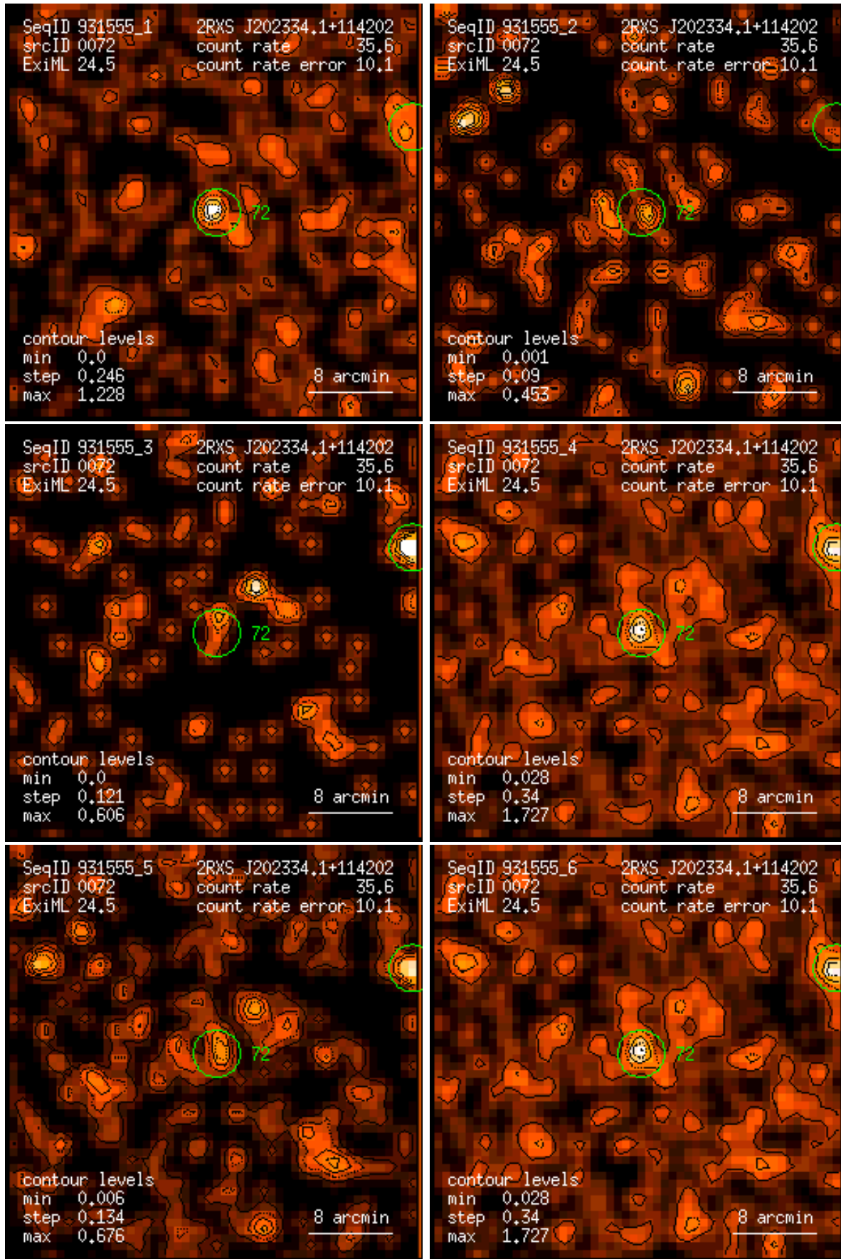
Figure 72: RASS 931555: detection 0072: band rate images, Gaussian filter: (1) PSPC channels 11 – 41, (2) 52 – 90, (3) 91 – 201, (4) 11 – 235, (5) 52 – 201, (6) 11 – 201. Broad band rates in counts/ks. Band rate contour levels in counts/ks/arcmin 2 .
