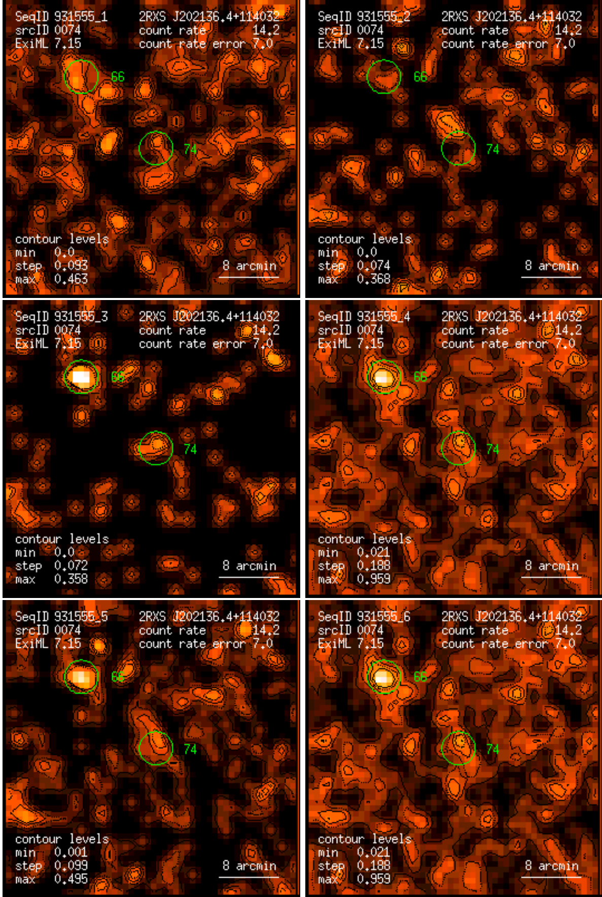
Figure 74: RASS 931555: detection 0074: band rate images, Gaussian filter: (1) PSPC channels 11 – 41, (2) 52 – 90, (3) 91 – 201, (4) 11 – 235, (5) 52 – 201, (6) 11 – 201. Broad band rates in counts/ks. Band rate contour levels in counts/ks/arcmin 2 .
