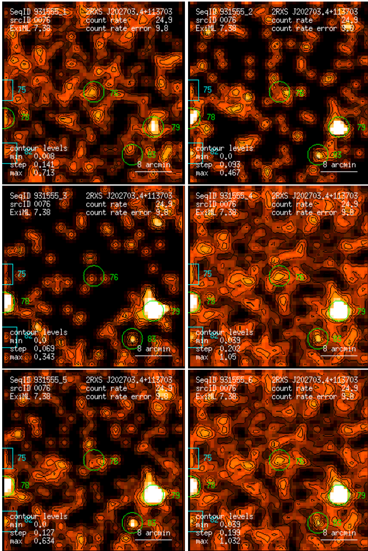
Figure 76: RASS 931555: detection 0076: band rate images, Gaussian filter: (1) PSPC channels 11 – 41, (2) 52 – 90, (3) 91 – 201, (4) 11 – 235, (5) 52 – 201, (6) 11 – 201. Broad band rates in counts/ks. Band rate contour levels in counts/ks/arcmin 2 .
