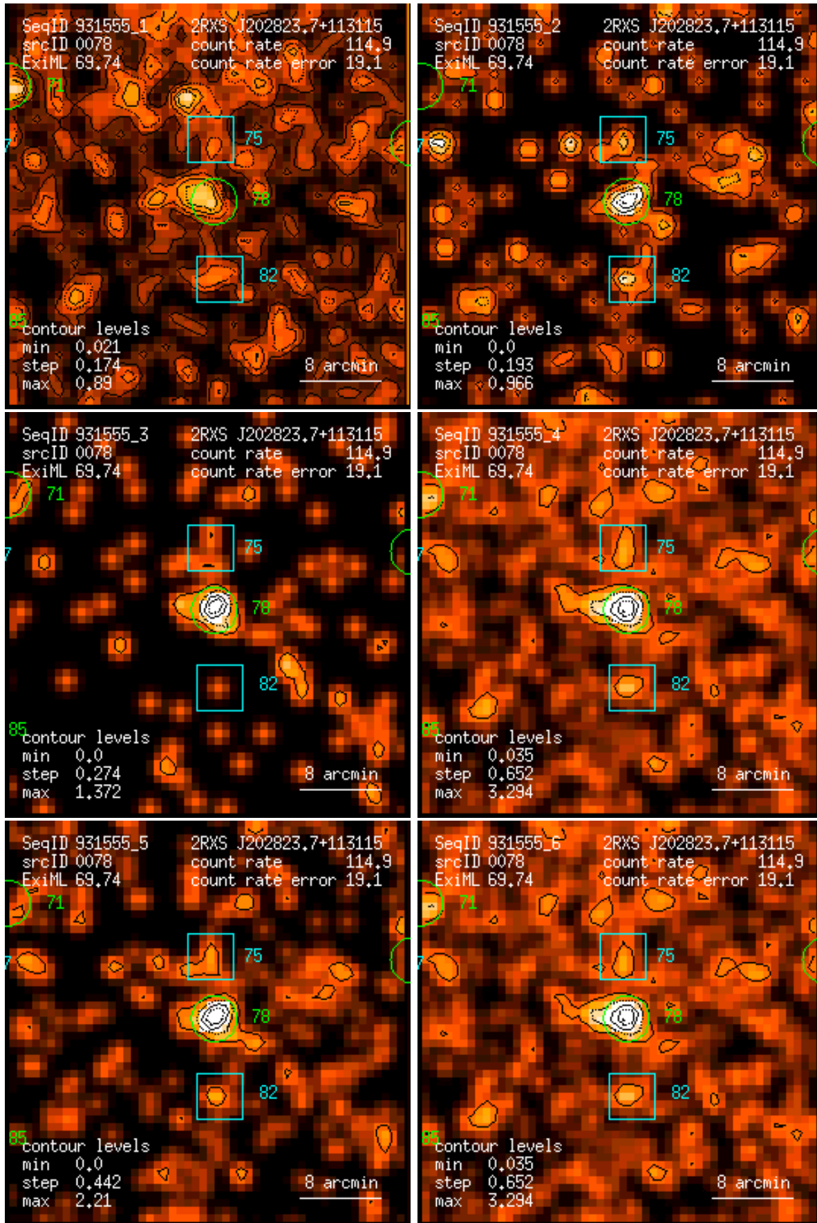
Figure 78: RASS 931555: detection 0078: band rate images, Gaussian filter: (1) PSPC channels 11 – 41, (2) 52 – 90, (3) 91 – 201, (4) 11 – 235, (5) 52 – 201, (6) 11 – 201. Broad band rates in counts/ks. Band rate contour levels in counts/ks/arcmin 2 .
