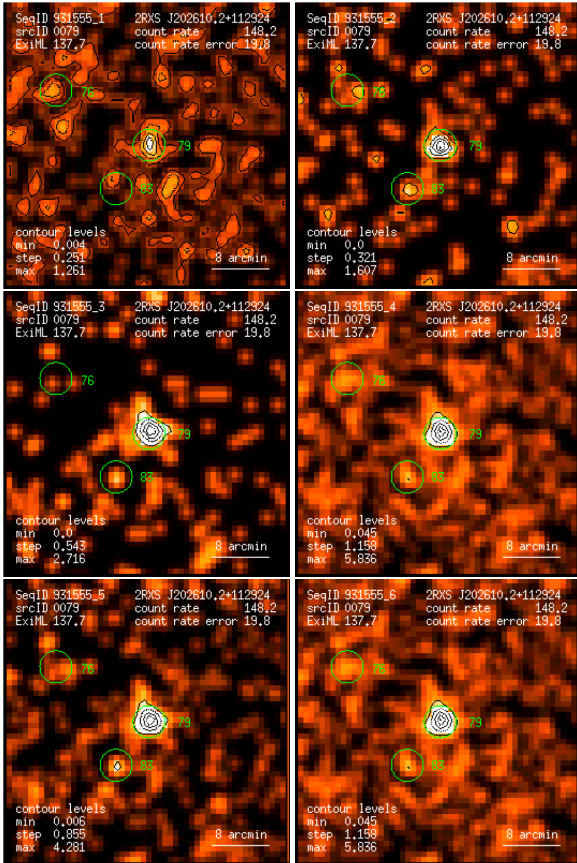
Figure 79: RASS 931555: detection 0079: band rate images, Gaussian filter: (1) PSPC channels 11 – 41, (2) 52 – 90, (3) 91 – 201, (4) 11 – 235, (5) 52 – 201, (6) 11 – 201. Broad band rates in counts/ks. Band rate contour levels in counts/ks/arcmin 2 .
