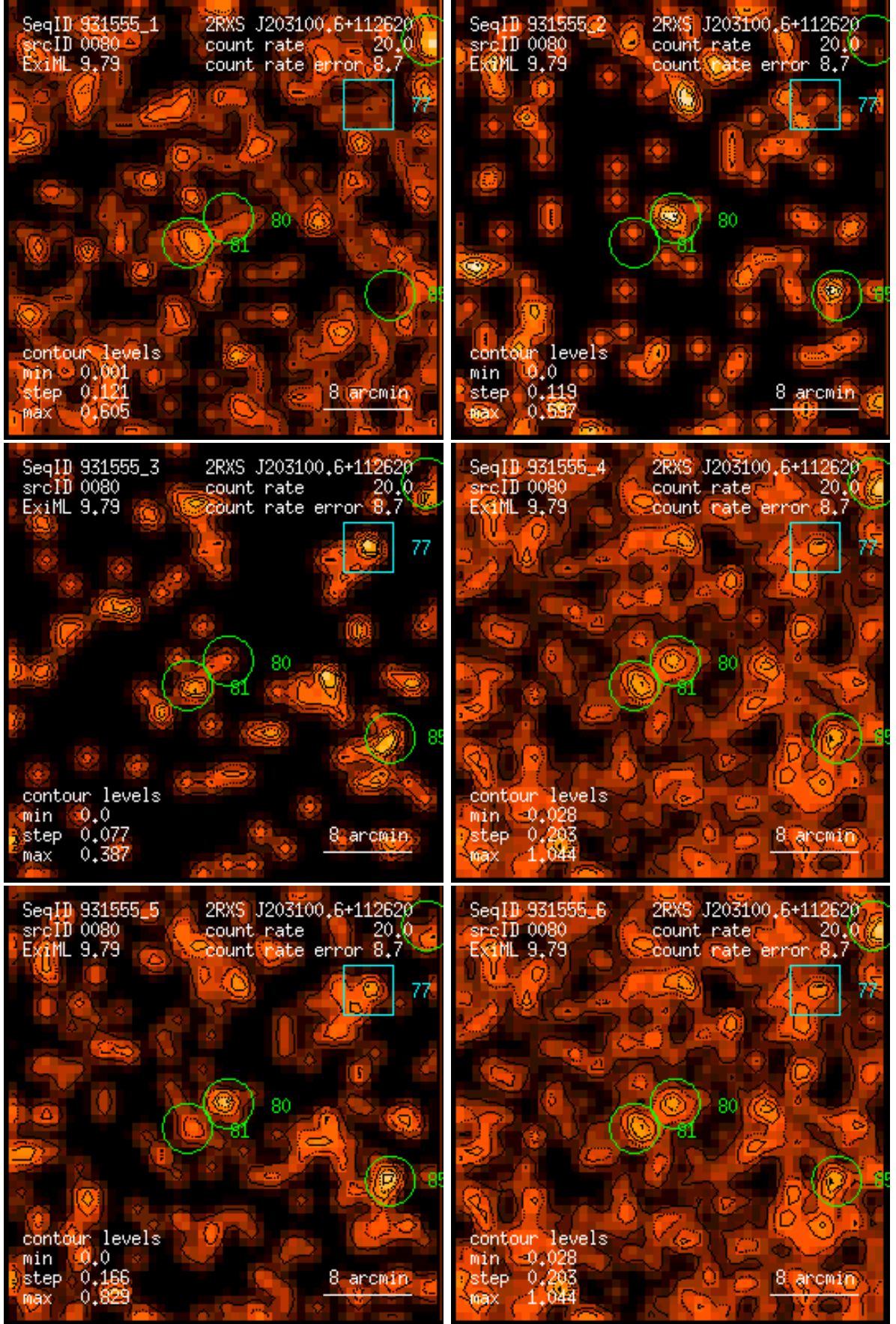
Figure 80: RASS 931555: detection 0080: band rate images, Gaussian filter: (1) PSPC channels 11 – 41, (2) 52 – 90, (3) 91 – 201, (4) 11 – 235, (5) 52 – 201, (6) 11 – 201. Broad band rates in counts/ks. Band rate contour levels in counts/ks/arcmin 2 .
