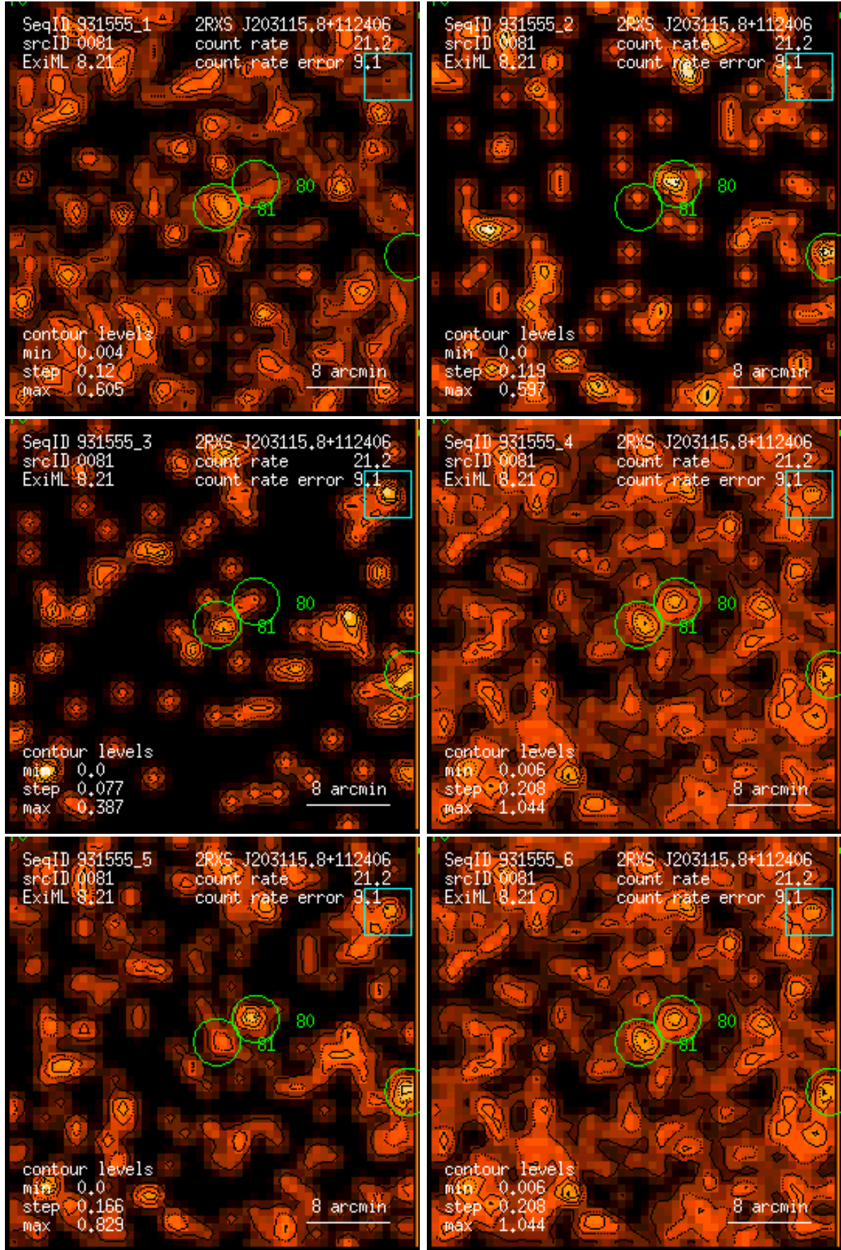
Figure 81: RASS 931555: detection 0081: band rate images, Gaussian filter: (1) PSPC channels 11 – 41, (2) 52 – 90, (3) 91 – 201, (4) 11 – 235, (5) 52 – 201, (6) 11 – 201. Broad band rates in counts/ks. Band rate contour levels in counts/ks/arcmin 2 .
