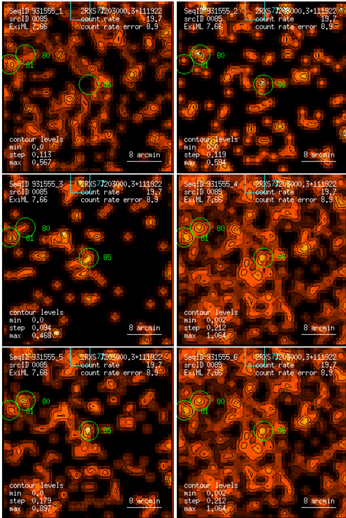
Figure 85: RASS 931555: detection 0085: band rate images, Gaussian filter: (1) PSPC channels 11 – 41, (2) 52 – 90, (3) 91 – 201, (4) 11 – 235, (5) 52 – 201, (6) 11 – 201. Broad band rates in counts/ks. Band rate contour levels in counts/ks/arcmin 2 .
