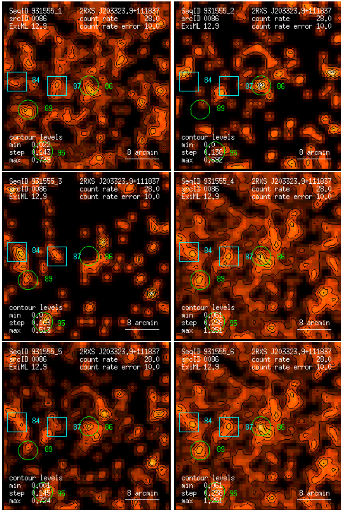
Figure 86: RASS 931555: detection 0086: band rate images, Gaussian filter: (1) PSPC channels 11 – 41, (2) 52 – 90, (3) 91 – 201, (4) 11 – 235, (5) 52 – 201, (6) 11 – 201. Broad band rates in counts/ks. Band rate contour levels in counts/ks/arcmin 2 .
