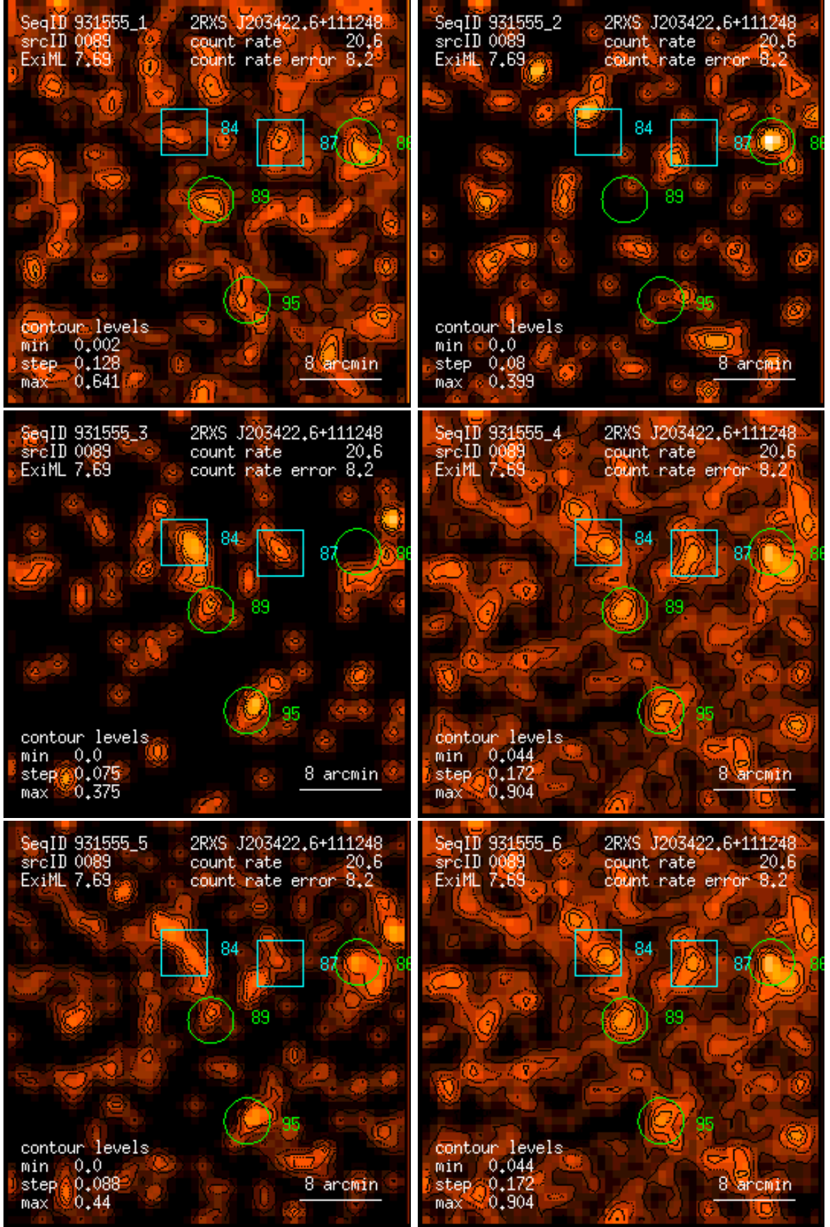
Figure 89: RASS 931555: detection 0089: band rate images, Gaussian filter: (1) PSPC channels 11 – 41, (2) 52 – 90, (3) 91 – 201, (4) 11 – 235, (5) 52 – 201, (6) 11 – 201. Broad band rates in counts/ks. Band rate contour levels in counts/ks/arcmin 2 .
