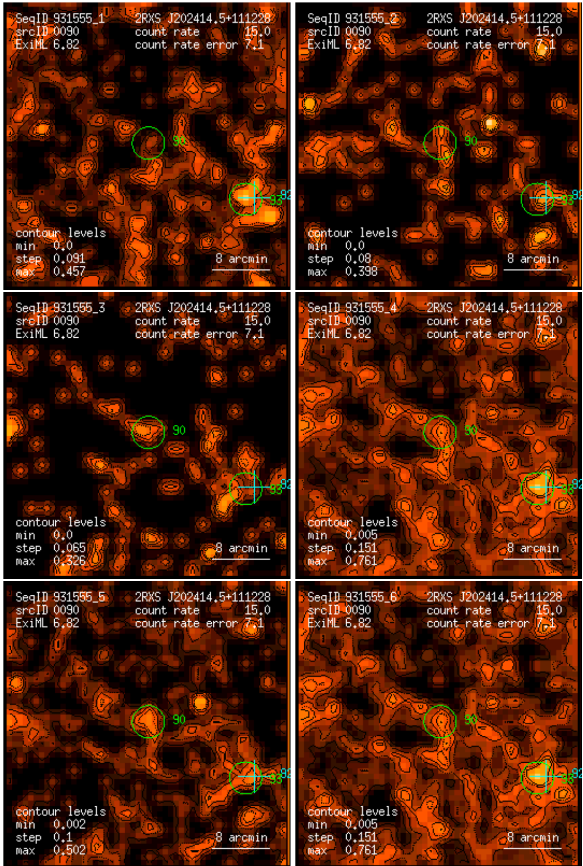
Figure 90: RASS 931555: detection 0090: band rate images, Gaussian filter: (1) PSPC channels 11 – 41, (2) 52 – 90, (3) 91 – 201, (4) 11 – 235, (5) 52 – 201, (6) 11 – 201. Broad band rates in counts/ks. Band rate contour levels in counts/ks/arcmin 2 .
