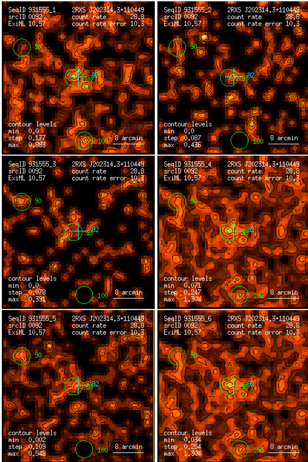
Figure 92: RASS 931555: detection 0092: band rate images, Gaussian filter: (1) PSPC channels 11 – 41, (2) 52 – 90, (3) 91 – 201, (4) 11 – 235, (5) 52 – 201, (6) 11 – 201. Broad band rates in counts/ks. Band rate contour levels in counts/ks/arcmin 2 .
