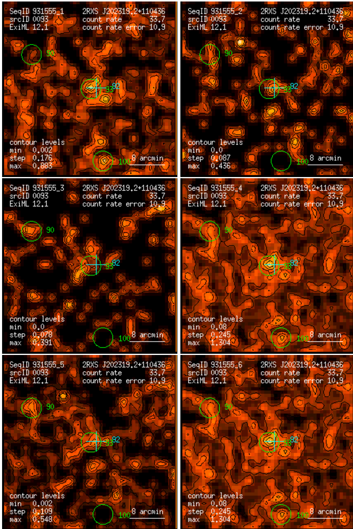
Figure 93: RASS 931555: detection 0093: band rate images, Gaussian filter: (1) PSPC channels 11 – 41, (2) 52 – 90, (3) 91 – 201, (4) 11 – 235, (5) 52 – 201, (6) 11 – 201. Broad band rates in counts/ks. Band rate contour levels in counts/ks/arcmin 2 .
