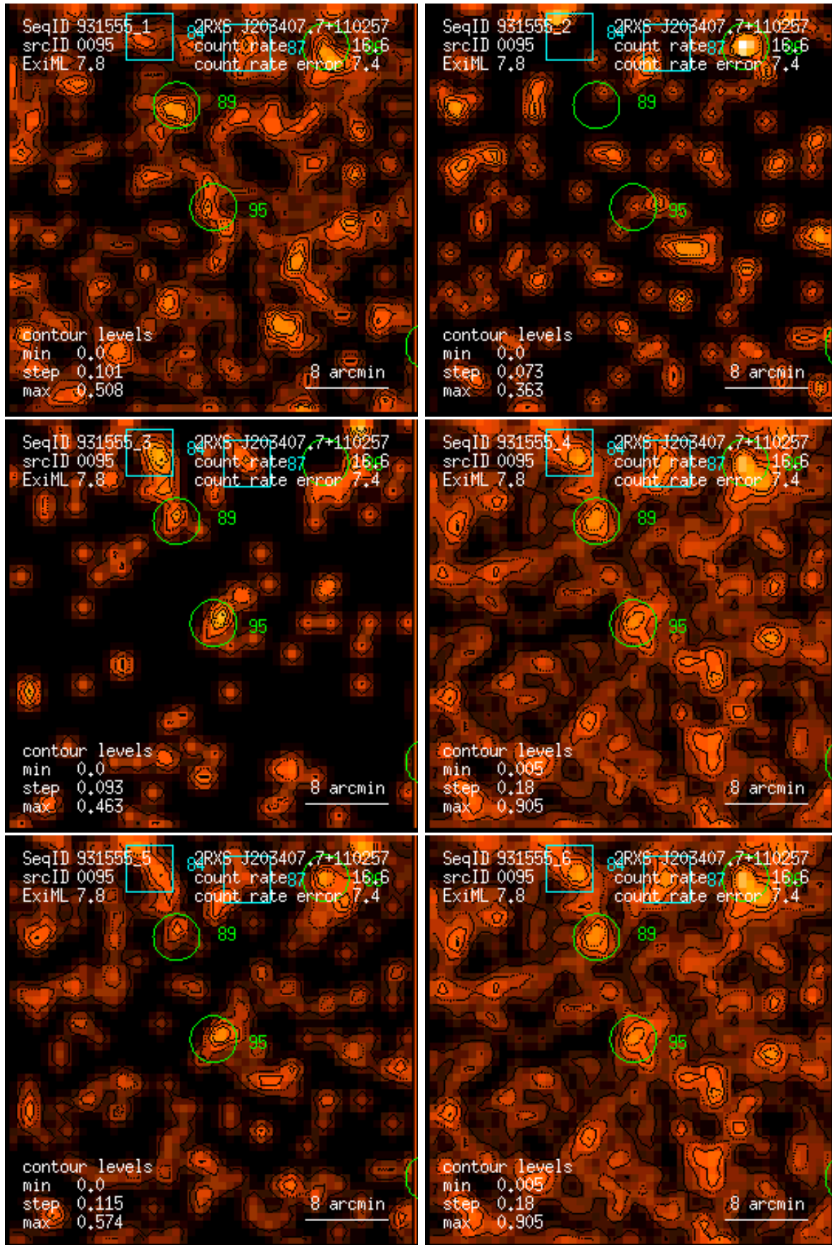
Figure 95: RASS 931555: detection 0095: band rate images, Gaussian filter: (1) PSPC channels 11 – 41, (2) 52 – 90, (3) 91 – 201, (4) 11 – 235, (5) 52 – 201, (6) 11 – 201. Broad band rates in counts/ks. Band rate contour levels in counts/ks/arcmin 2 .
