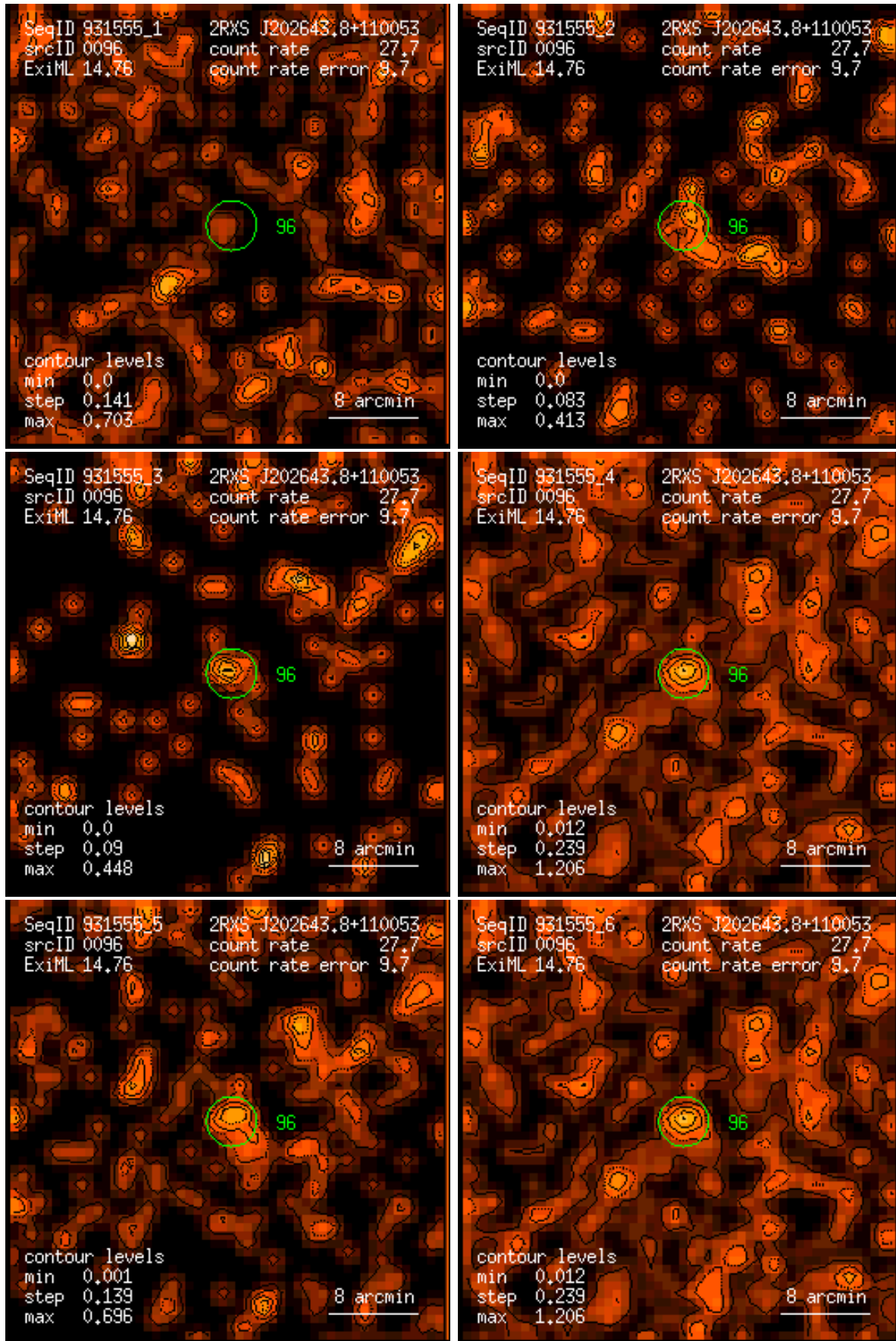
Figure 96: RASS 931555: detection 0096: band rate images, Gaussian filter: (1) PSPC channels 11 – 41, (2) 52 – 90, (3) 91 – 201, (4) 11 – 235, (5) 52 – 201, (6) 11 – 201. Broad band rates in counts/ks. Band rate contour levels in counts/ks/arcmin 2 .
