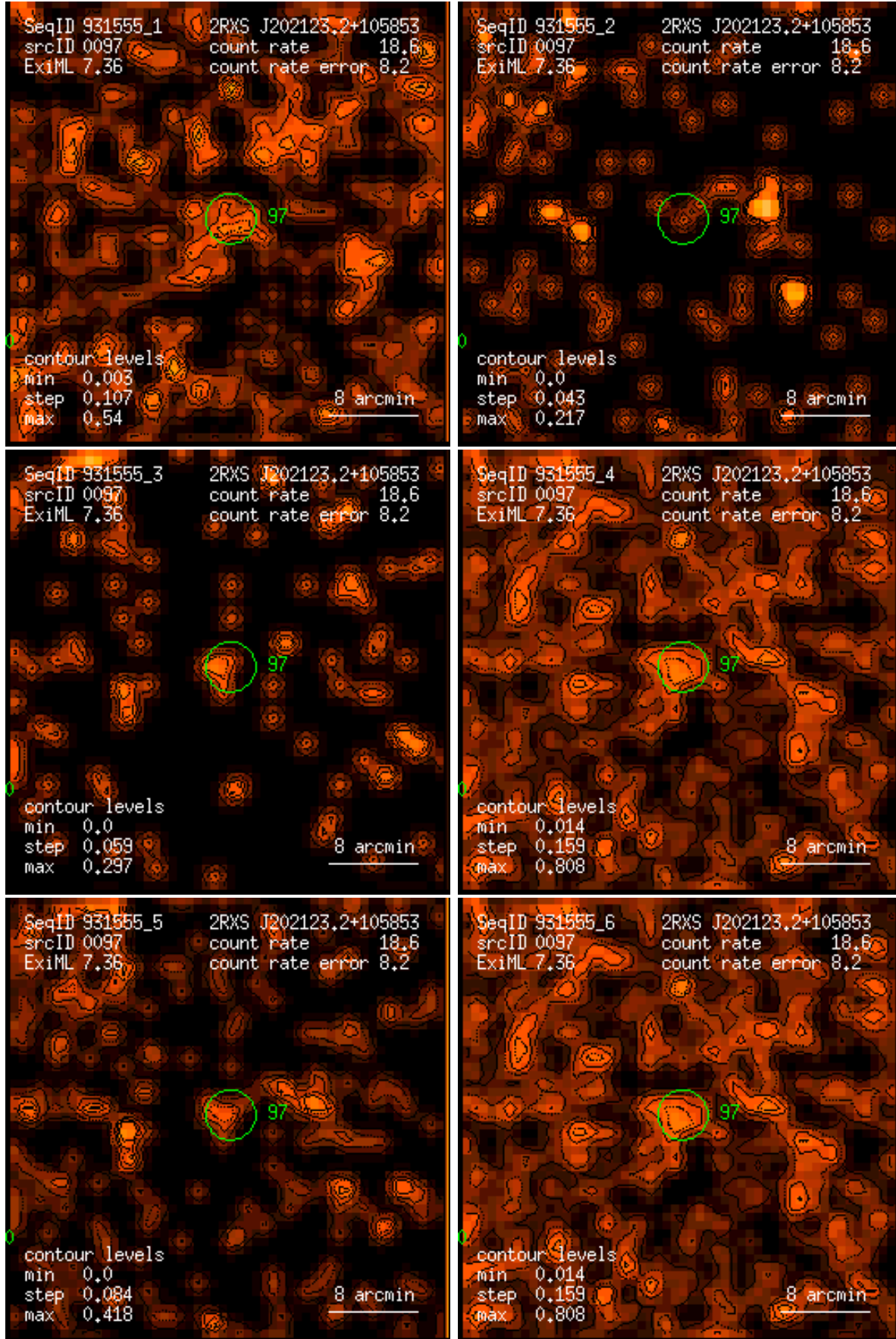
Figure 97: RASS 931555: detection 0097: band rate images, Gaussian filter: (1) PSPC channels 11 – 41, (2) 52 – 90, (3) 91 – 201, (4) 11 – 235, (5) 52 – 201, (6) 11 – 201. Broad band rates in counts/ks. Band rate contour levels in counts/ks/arcmin 2 .
