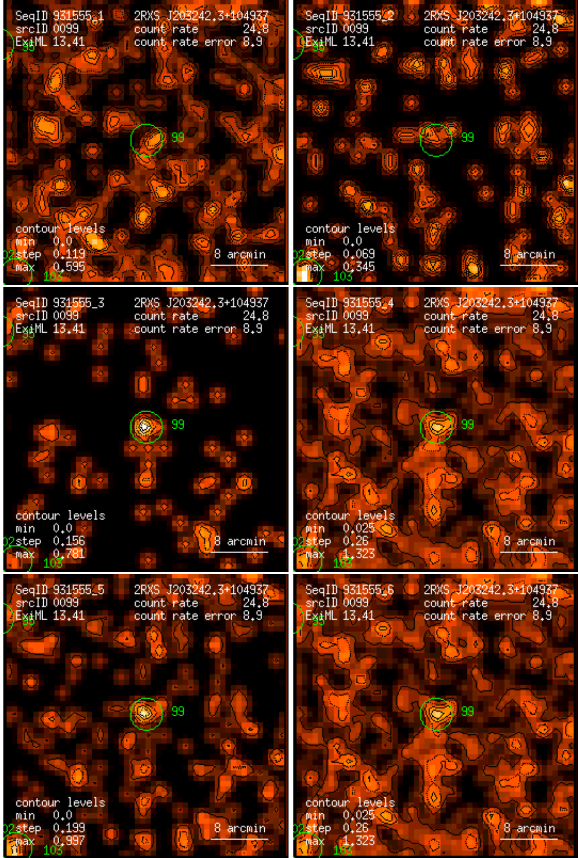
Figure 99: RASS 931555: detection 0099: band rate images, Gaussian filter: (1) PSPC channels 11 – 41, (2) 52 – 90, (3) 91 – 201, (4) 11 – 235, (5) 52 – 201, (6) 11 – 201. Broad band rates in counts/ks. Band rate contour levels in counts/ks/arcmin 2 .
