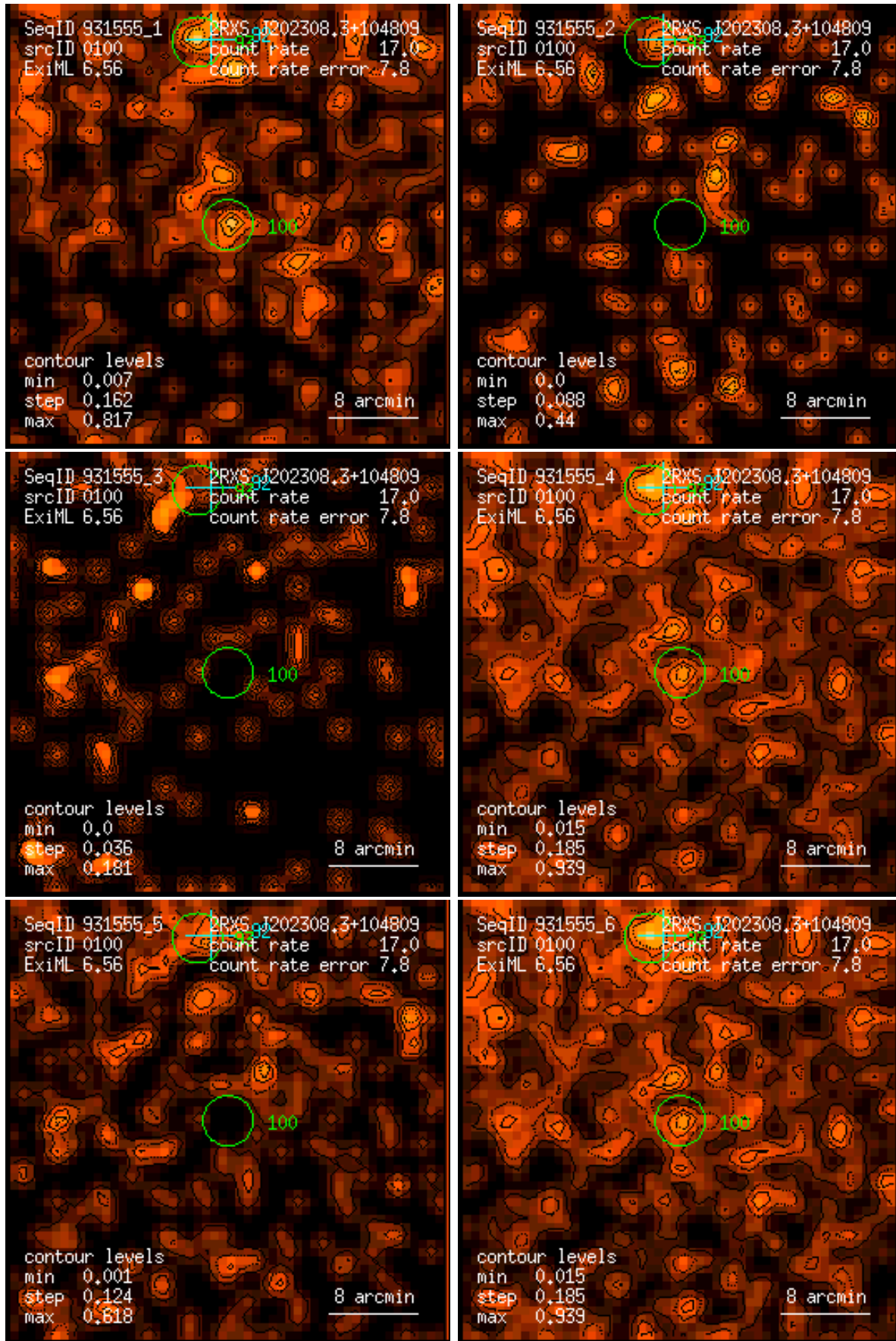
Figure 100: RASS 931555: detection 0100: band rate images, Gaussian filter: (1) PSPC channels 11 – 41, (2) 52 – 90, (3) 91 – 201, (4) 11 – 235, (5) 52 – 201, (6) 11 – 201. Broad band rates in counts/ks. Band rate contour levels in counts/ks/arcmin 2 .
