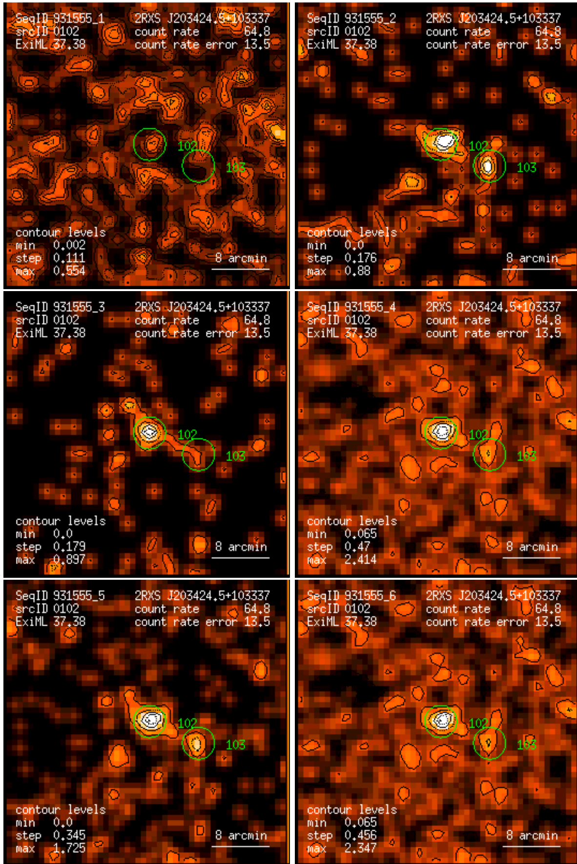
Figure 102: RASS 931555: detection 0102: band rate images, Gaussian filter: (1) PSPC channels 11 – 41, (2) 52 – 90, (3) 91 – 201, (4) 11 – 235, (5) 52 – 201, (6) 11 – 201. Broad band rates in counts/ks. Band rate contour levels in counts/ks/arcmin 2 .
