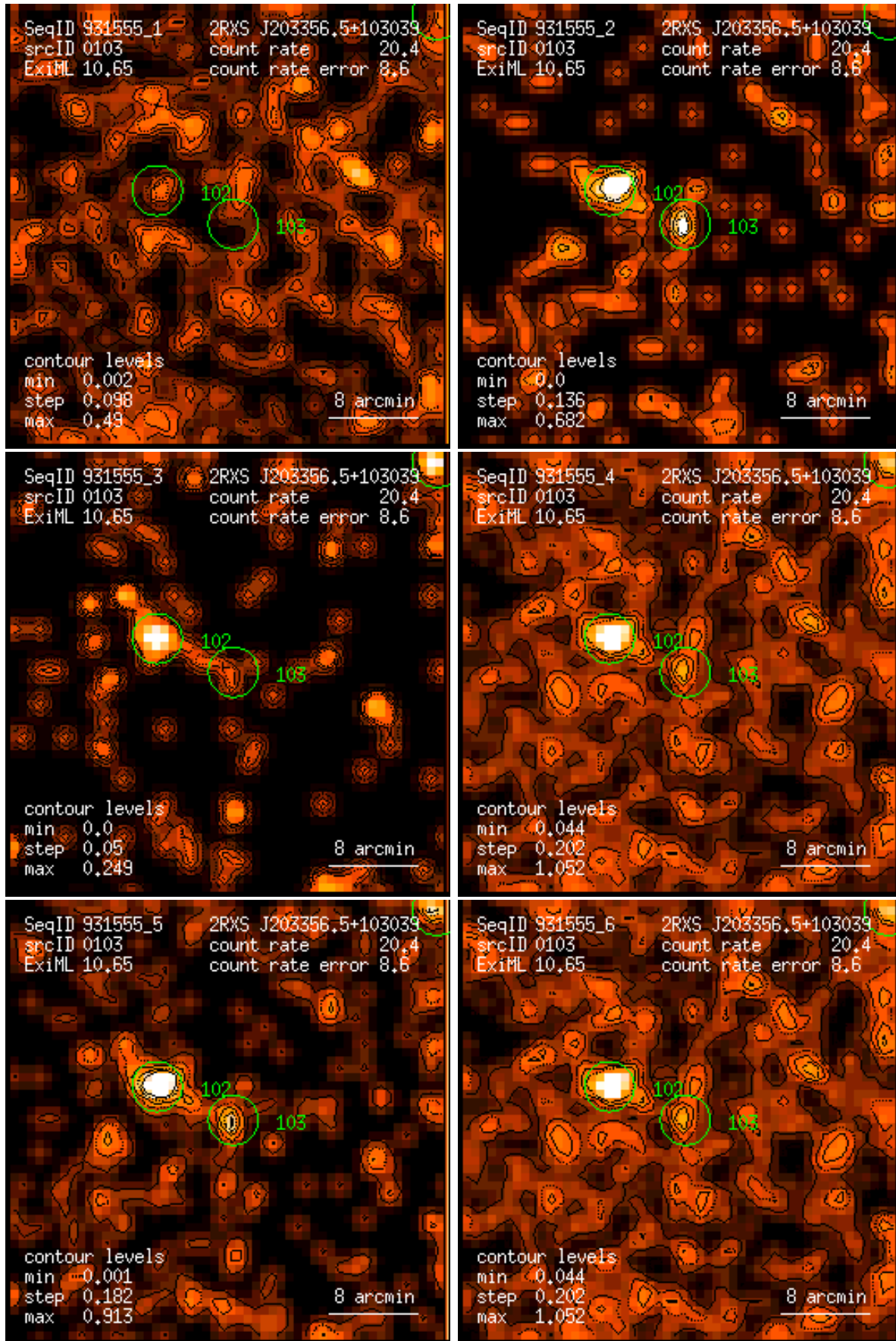
Figure 103: RASS 931555: detection 0103: band rate images, Gaussian filter: (1) PSPC channels 11 – 41, (2) 52 – 90, (3) 91 – 201, (4) 11 – 235, (5) 52 – 201, (6) 11 – 201. Broad band rates in counts/ks. Band rate contour levels in counts/ks/arcmin 2 .
