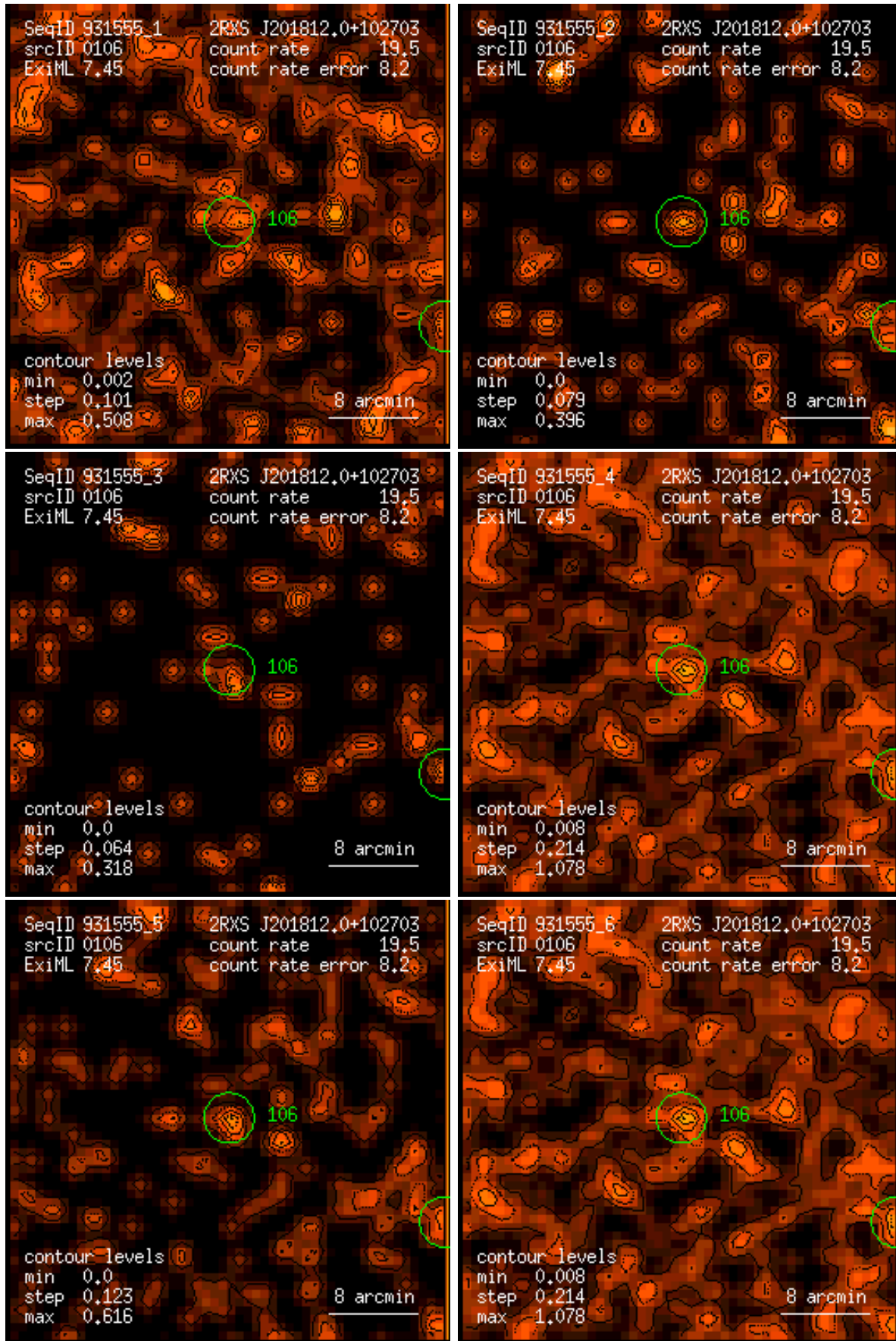
Figure 106: RASS 931555: detection 0106: band rate images, Gaussian filter: (1) PSPC channels 11 – 41, (2) 52 – 90, (3) 91 – 201, (4) 11 – 235, (5) 52 – 201, (6) 11 – 201. Broad band rates in counts/ks. Band rate contour levels in counts/ks/arcmin 2 .
