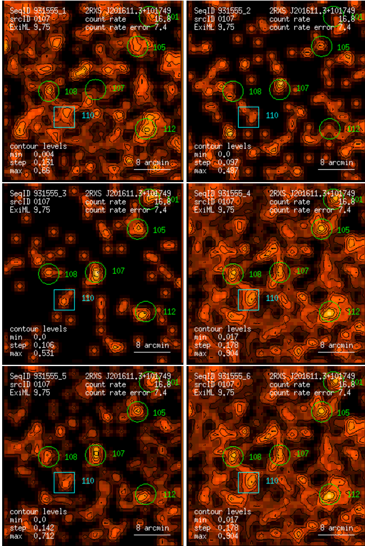
Figure 107: RASS 931555: detection 0107: band rate images, Gaussian filter: (1) PSPC channels 11 – 41, (2) 52 – 90, (3) 91 – 201, (4) 11 – 235, (5) 52 – 201, (6) 11 – 201. Broad band rates in counts/ks. Band rate contour levels in counts/ks/arcmin 2 .
