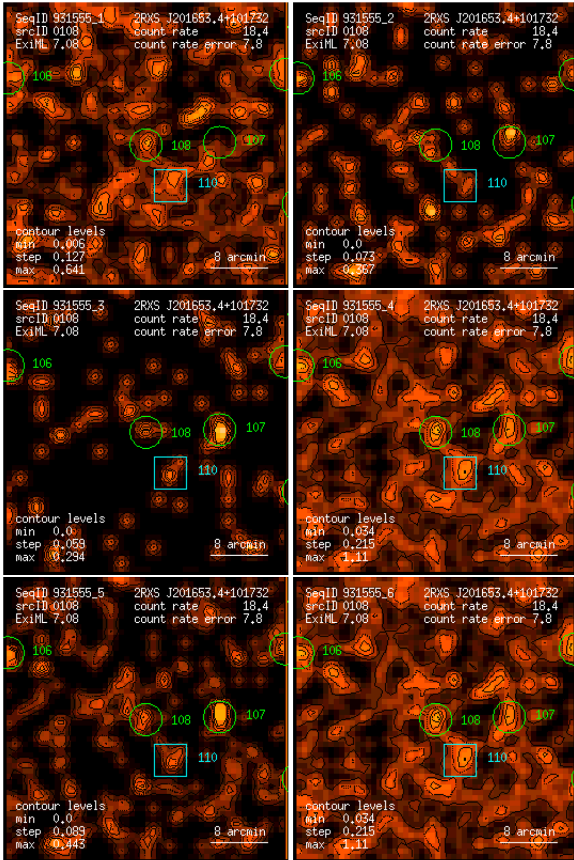
Figure 108: RASS 931555: detection 0108: band rate images, Gaussian filter: (1) PSPC channels 11 – 41, (2) 52 – 90, (3) 91 – 201, (4) 11 – 235, (5) 52 – 201, (6) 11 – 201. Broad band rates in counts/ks. Band rate contour levels in counts/ks/arcmin 2 .
