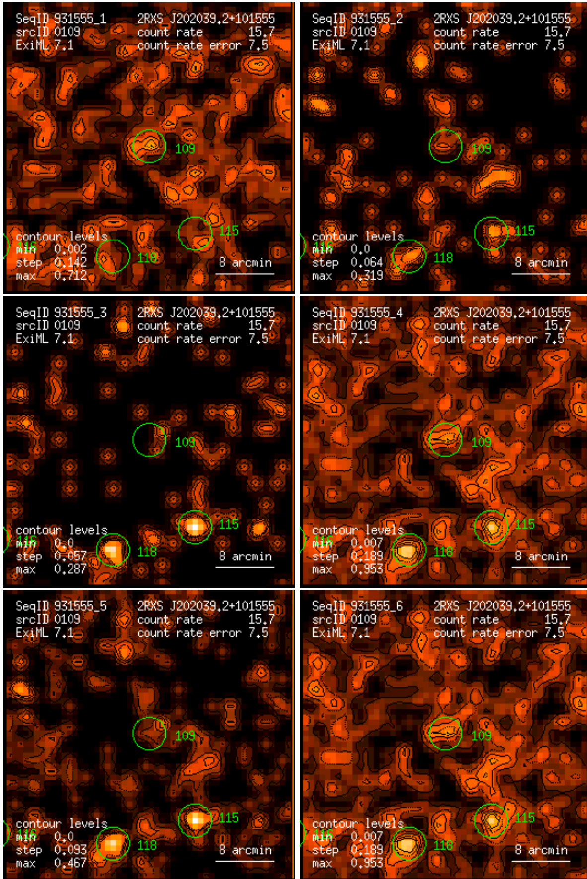
Figure 109: RASS 931555: detection 0109: band rate images, Gaussian filter: (1) PSPC channels 11 – 41, (2) 52 – 90, (3) 91 – 201, (4) 11 – 235, (5) 52 – 201, (6) 11 – 201. Broad band rates in counts/ks. Band rate contour levels in counts/ks/arcmin 2 .
