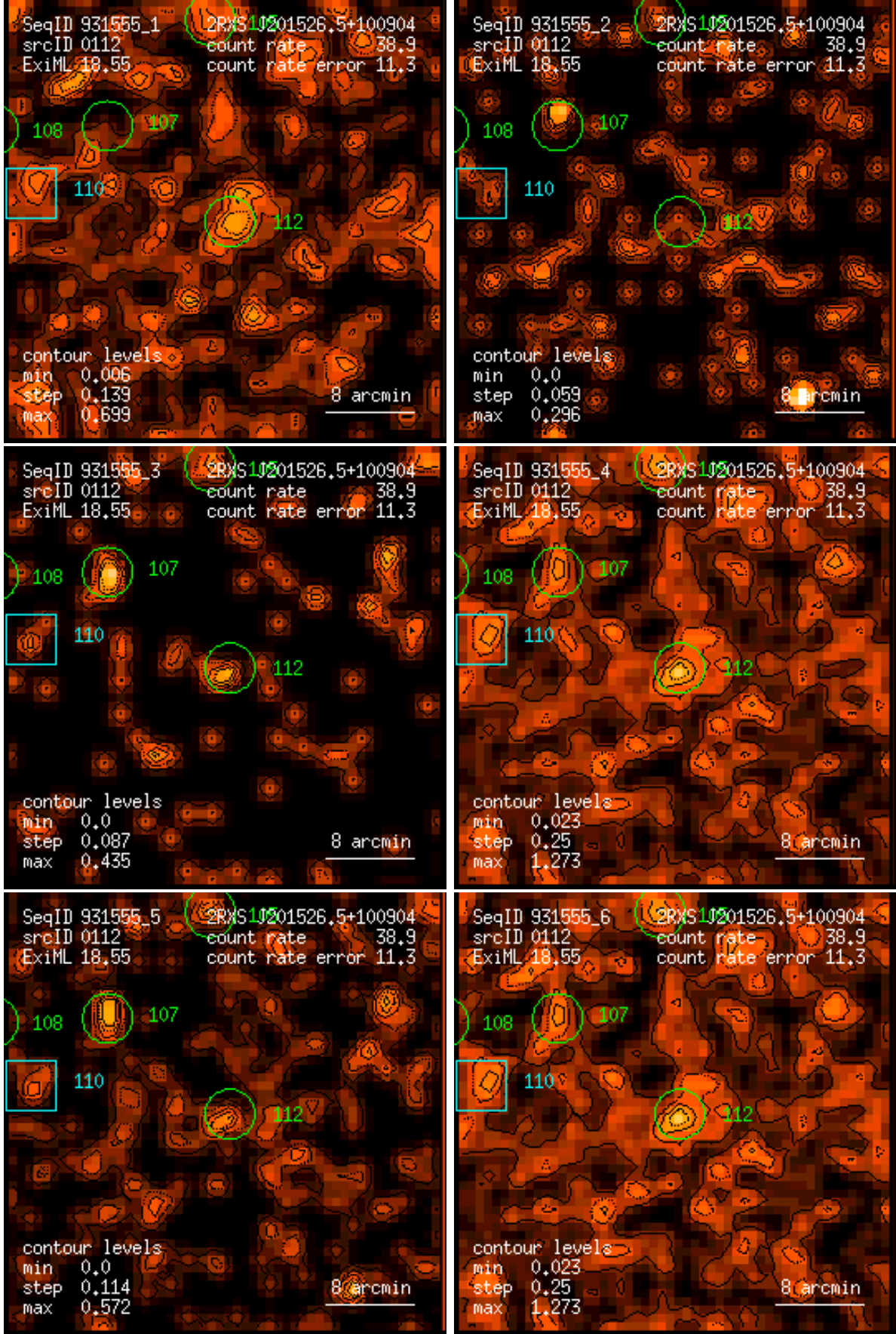
Figure 112: RASS 931555: detection 0112: band rate images, Gaussian filter: (1) PSPC channels 11 – 41, (2) 52 – 90, (3) 91 – 201, (4) 11 – 235, (5) 52 – 201, (6) 11 – 201. Broad band rates in counts/ks. Band rate contour levels in counts/ks/arcmin 2 .
