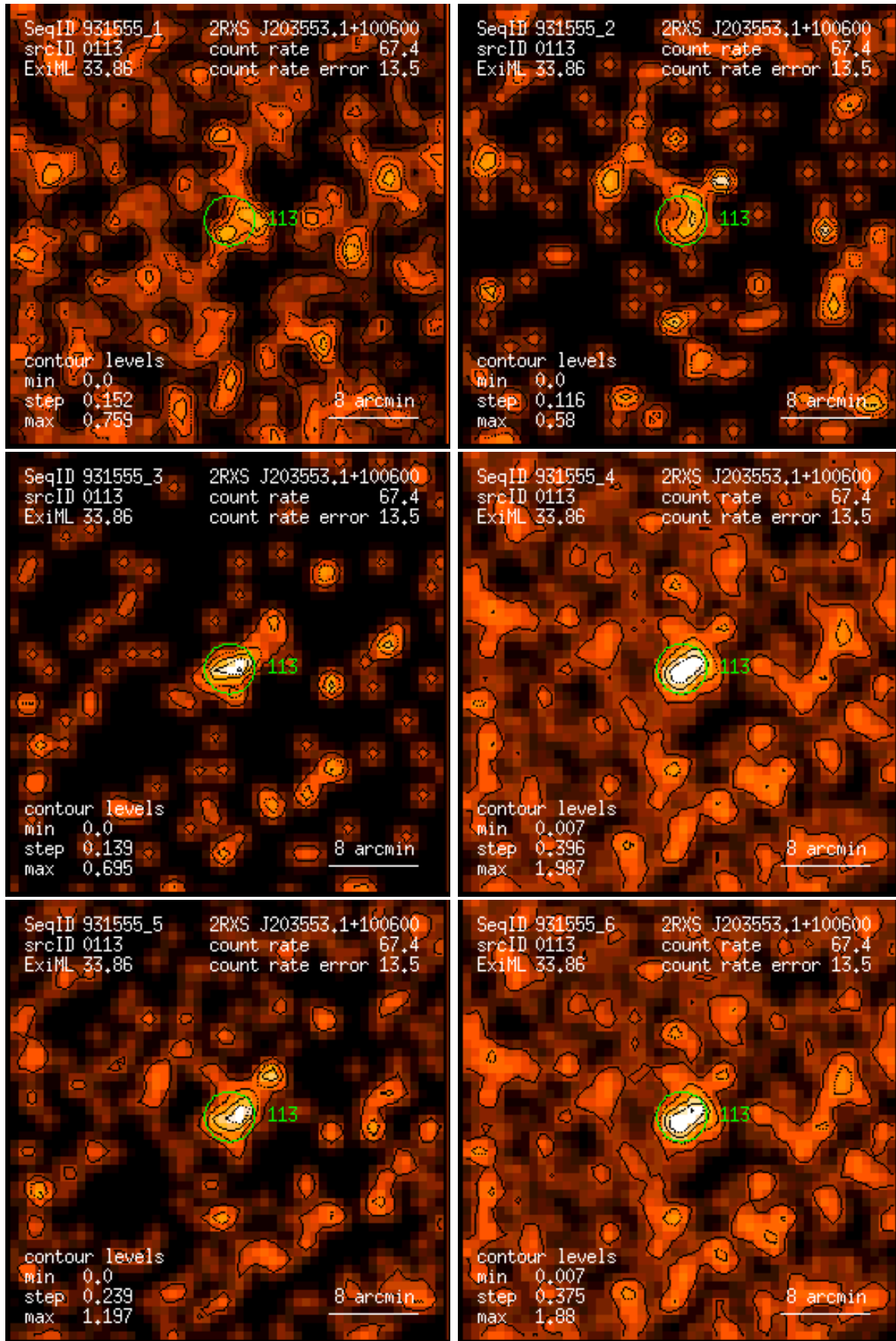
Figure 113: RASS 931555: detection 0113: band rate images, Gaussian filter: (1) PSPC channels 11 – 41, (2) 52 – 90, (3) 91 – 201, (4) 11 – 235, (5) 52 – 201, (6) 11 – 201. Broad band rates in counts/ks. Band rate contour levels in counts/ks/arcmin 2 .
