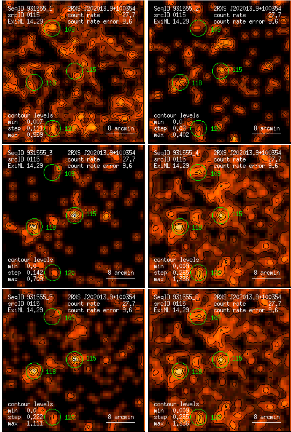
Figure 115: RASS 931555: detection 0115: band rate images, Gaussian filter: (1) PSPC channels 11 – 41, (2) 52 – 90, (3) 91 – 201, (4) 11 – 235, (5) 52 – 201, (6) 11 – 201. Broad band rates in counts/ks. Band rate contour levels in counts/ks/arcmin 2 .
