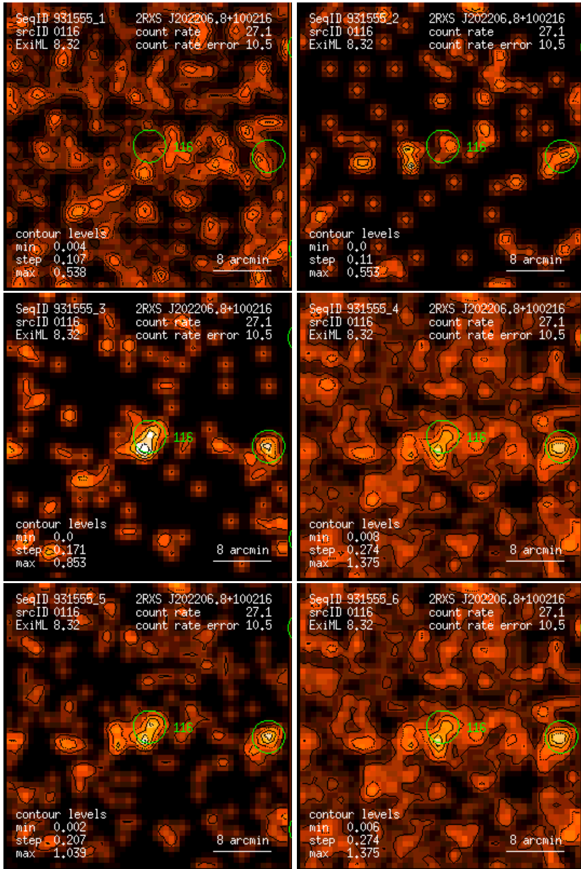
Figure 116: RASS 931555: detection 0116: band rate images, Gaussian filter: (1) PSPC channels 11 – 41, (2) 52 – 90, (3) 91 – 201, (4) 11 – 235, (5) 52 – 201, (6) 11 – 201. Broad band rates in counts/ks. Band rate contour levels in counts/ks/arcmin 2 .
