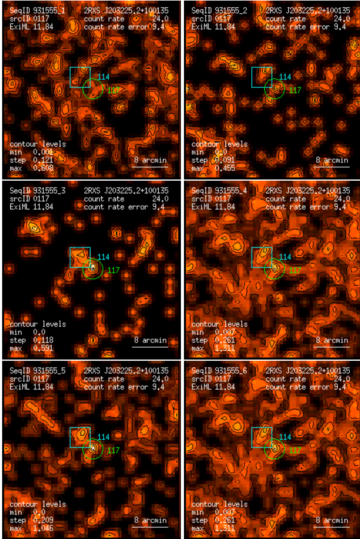
Figure 117: RASS 931555: detection 0117: band rate images, Gaussian filter: (1) PSPC channels 11 – 41, (2) 52 – 90, (3) 91 – 201, (4) 11 – 235, (5) 52 – 201, (6) 11 – 201. Broad band rates in counts/ks. Band rate contour levels in counts/ks/arcmin 2 .
