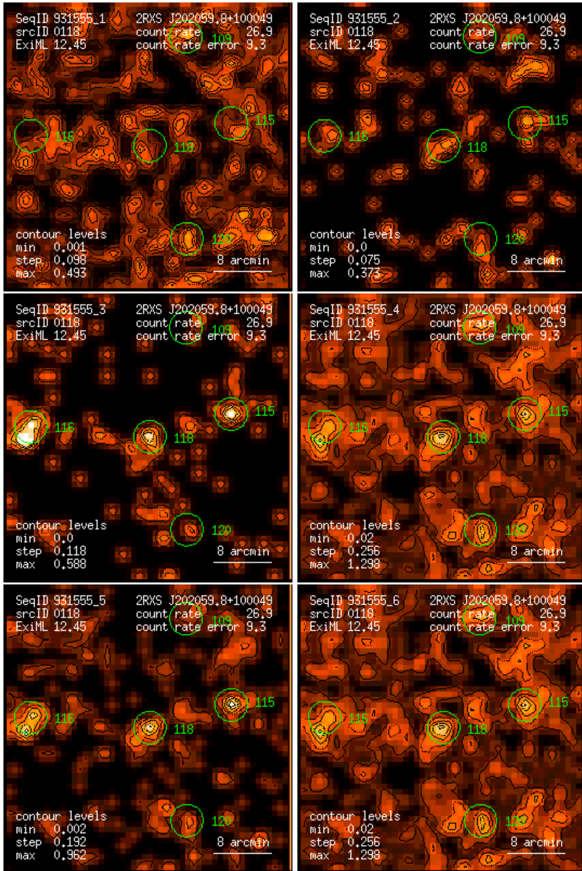
Figure 118: RASS 931555: detection 0118: band rate images, Gaussian filter: (1) PSPC channels 11 – 41, (2) 52 – 90, (3) 91 – 201, (4) 11 – 235, (5) 52 – 201, (6) 11 – 201. Broad band rates in counts/ks. Band rate contour levels in counts/ks/arcmin 2 .
