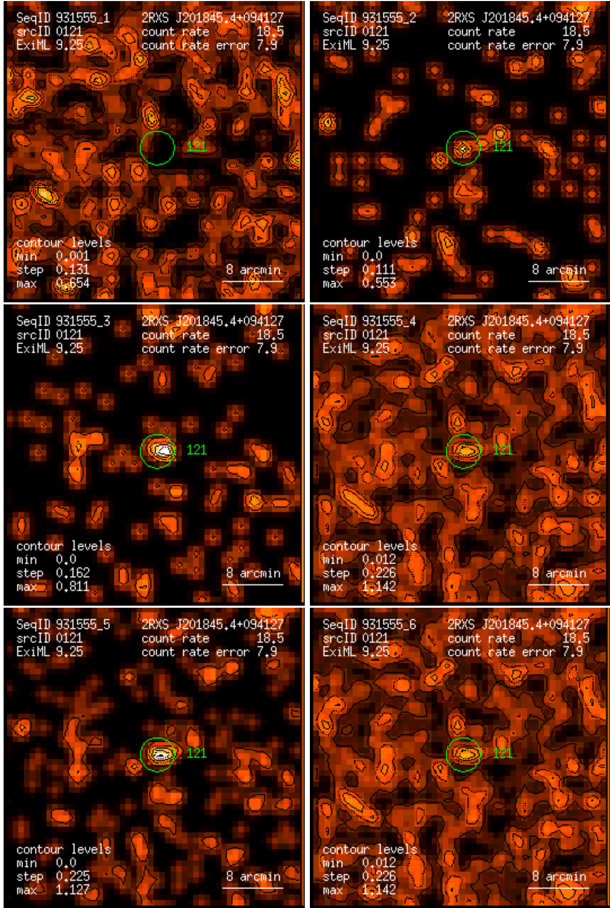
Figure 121: RASS 931555: detection 0121: band rate images, Gaussian filter: (1) PSPC channels 11 – 41, (2) 52 – 90, (3) 91 – 201, (4) 11 – 235, (5) 52 – 201, (6) 11 – 201. Broad band rates in counts/ks. Band rate contour levels in counts/ks/arcmin 2 .
