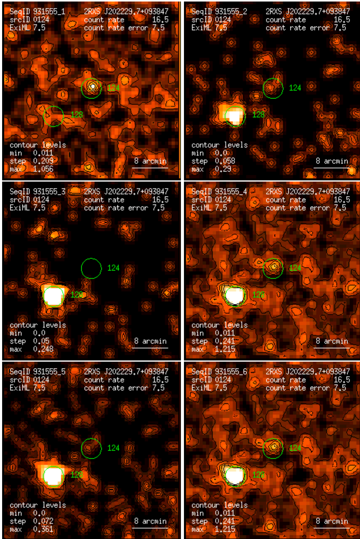
Figure 124: RASS 931555: detection 0124: band rate images, Gaussian filter: (1) PSPC channels 11 – 41, (2) 52 – 90, (3) 91 – 201, (4) 11 – 235, (5) 52 – 201, (6) 11 – 201. Broad band rates in counts/ks. Band rate contour levels in counts/ks/arcmin 2 .
