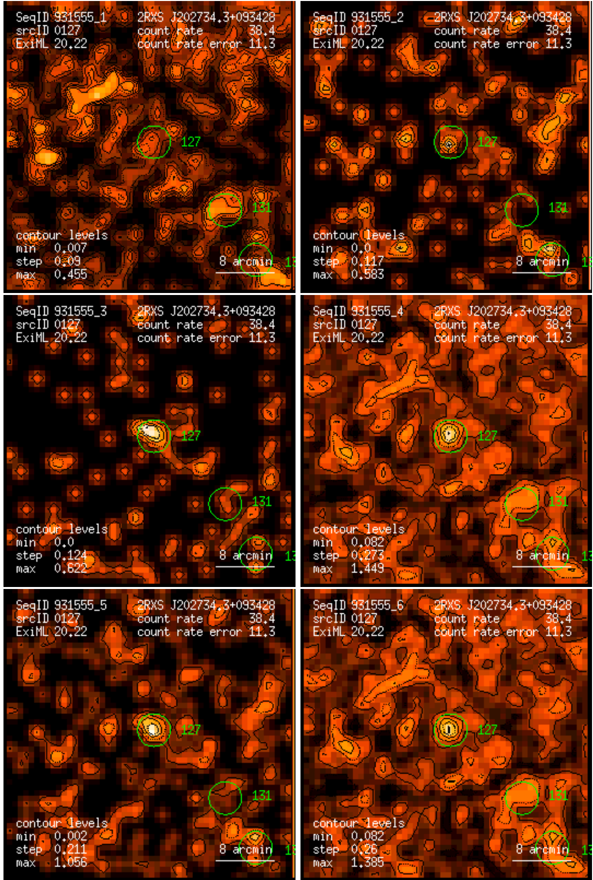
Figure 127: RASS 931555: detection 0127: band rate images, Gaussian filter: (1) PSPC channels 11 – 41, (2) 52 – 90, (3) 91 – 201, (4) 11 – 235, (5) 52 – 201, (6) 11 – 201. Broad band rates in counts/ks. Band rate contour levels in counts/ks/arcmin 2 .
