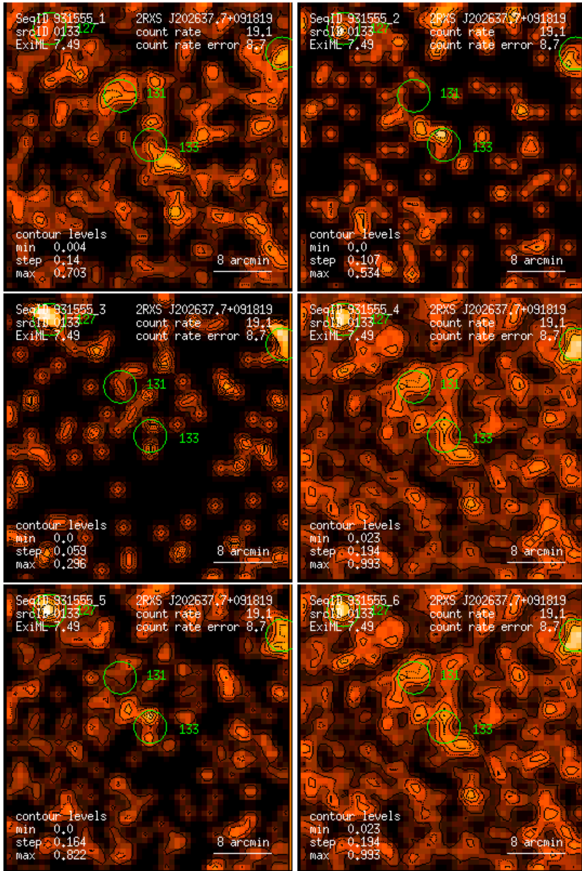
Figure 133: RASS 931555: detection 0133: band rate images, Gaussian filter: (1) PSPC channels 11 – 41, (2) 52 – 90, (3) 91 – 201, (4) 11 – 235, (5) 52 – 201, (6) 11 – 201. Broad band rates in counts/ks. Band rate contour levels in counts/ks/arcmin 2 .
